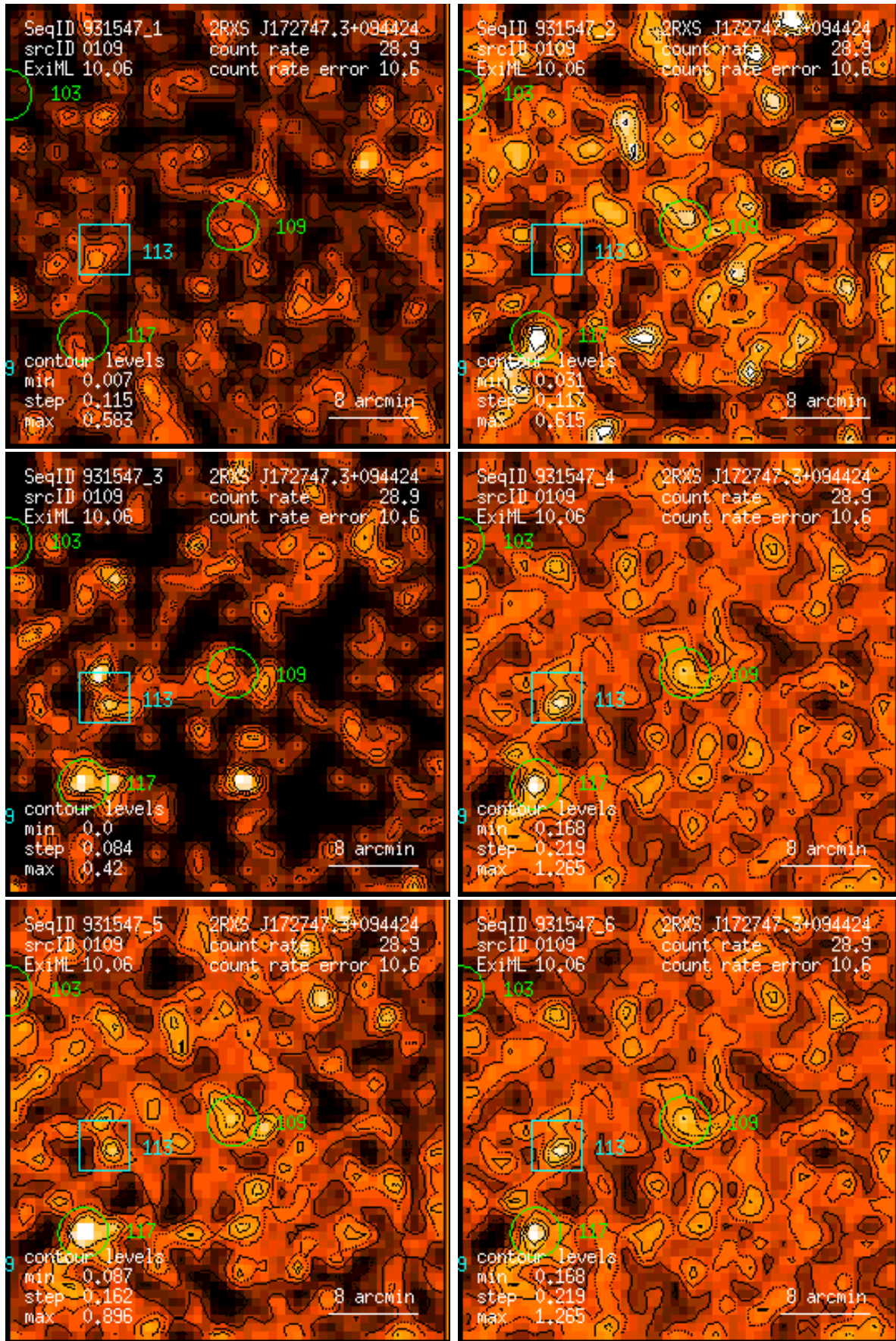
Figure 109: RASS 931547: detection 0109: band rate images, Gaussian filter: (1) PSPC channels 11 – 41, (2) 52 – 90, (3) 91 – 201, (4) 11 – 235, (5) 52 – 201, (6) 11 – 201. Broad band rates in counts/ks. Band rate contour levels in counts/ks/arcmin 2 .
