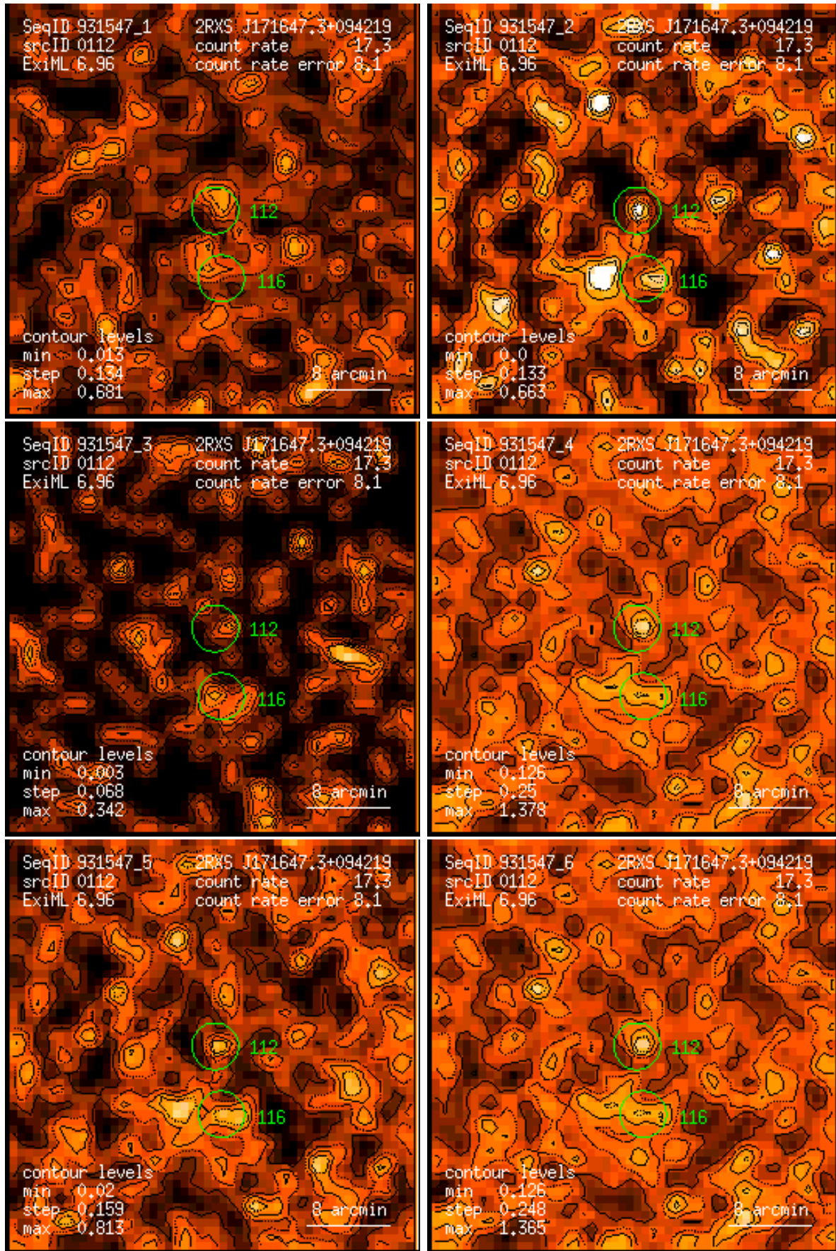
Figure 112: RASS 931547: detection 0112: band rate images, Gaussian filter: (1) PSPC channels 11 – 41, (2) 52 – 90, (3) 91 – 201, (4) 11 – 235, (5) 52 – 201, (6) 11 – 201. Broad band rates in counts/ks. Band rate contour levels in counts/ks/arcmin 2 .
