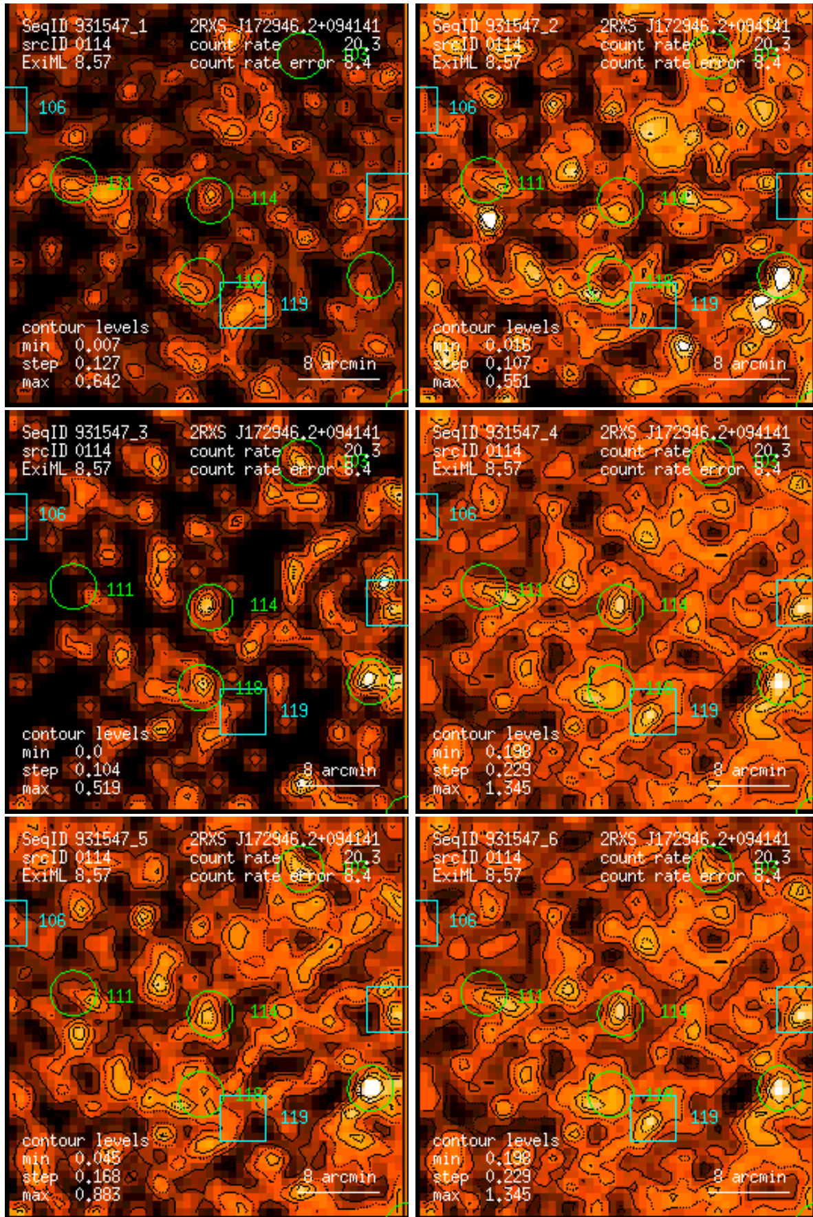
Figure 114: RASS 931547: detection 0114: band rate images, Gaussian filter: (1) PSPC channels 11 – 41, (2) 52 – 90, (3) 91 – 201, (4) 11 – 235, (5) 52 – 201, (6) 11 – 201. Broad band rates in counts/ks. Band rate contour levels in counts/ks/arcmin 2 .
