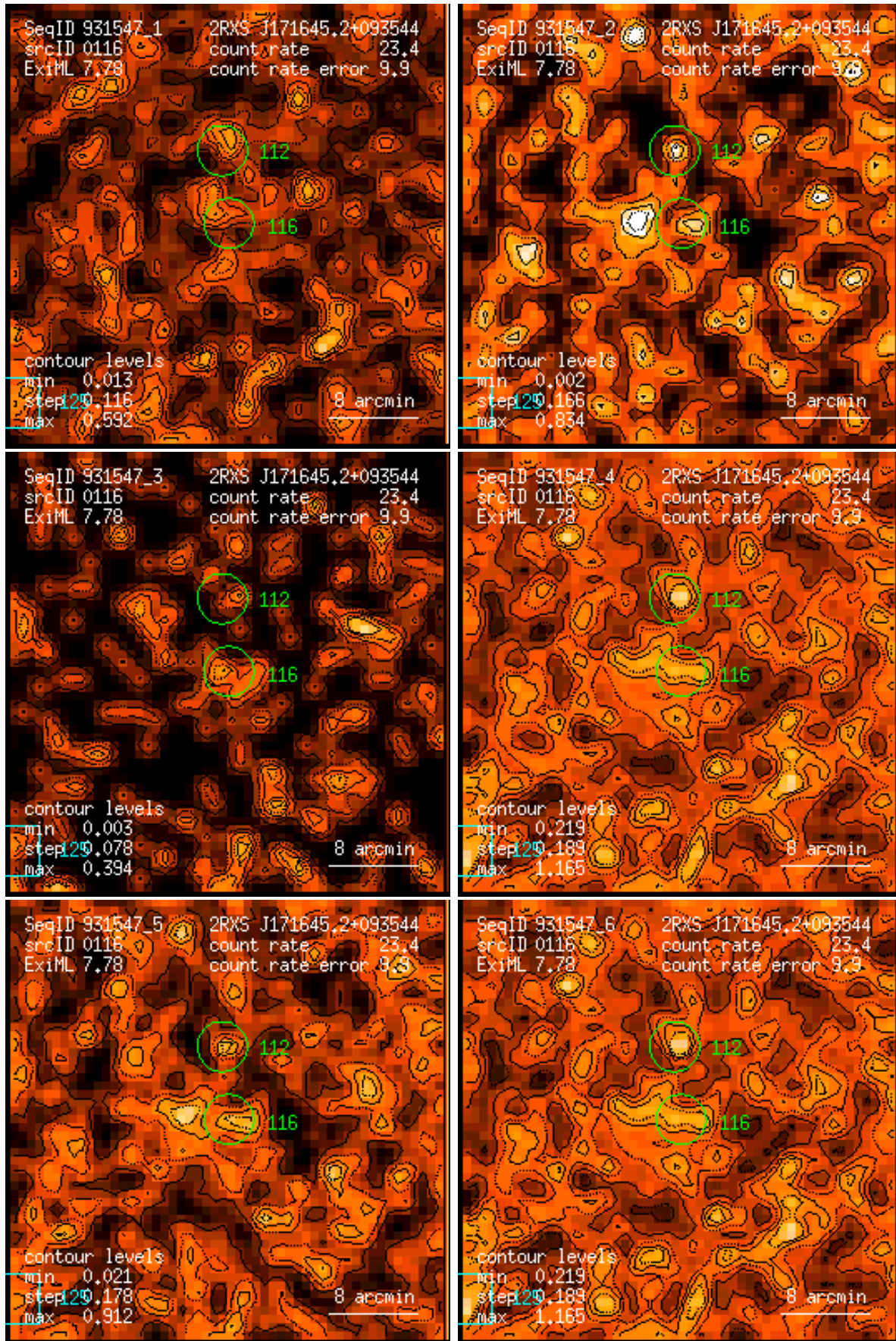
Figure 116: RASS 931547: detection 0116: band rate images, Gaussian filter: (1) PSPC channels 11 – 41, (2) 52 – 90, (3) 91 – 201, (4) 11 – 235, (5) 52 – 201, (6) 11 – 201. Broad band rates in counts/ks. Band rate contour levels in counts/ks/arcmin 2 .
