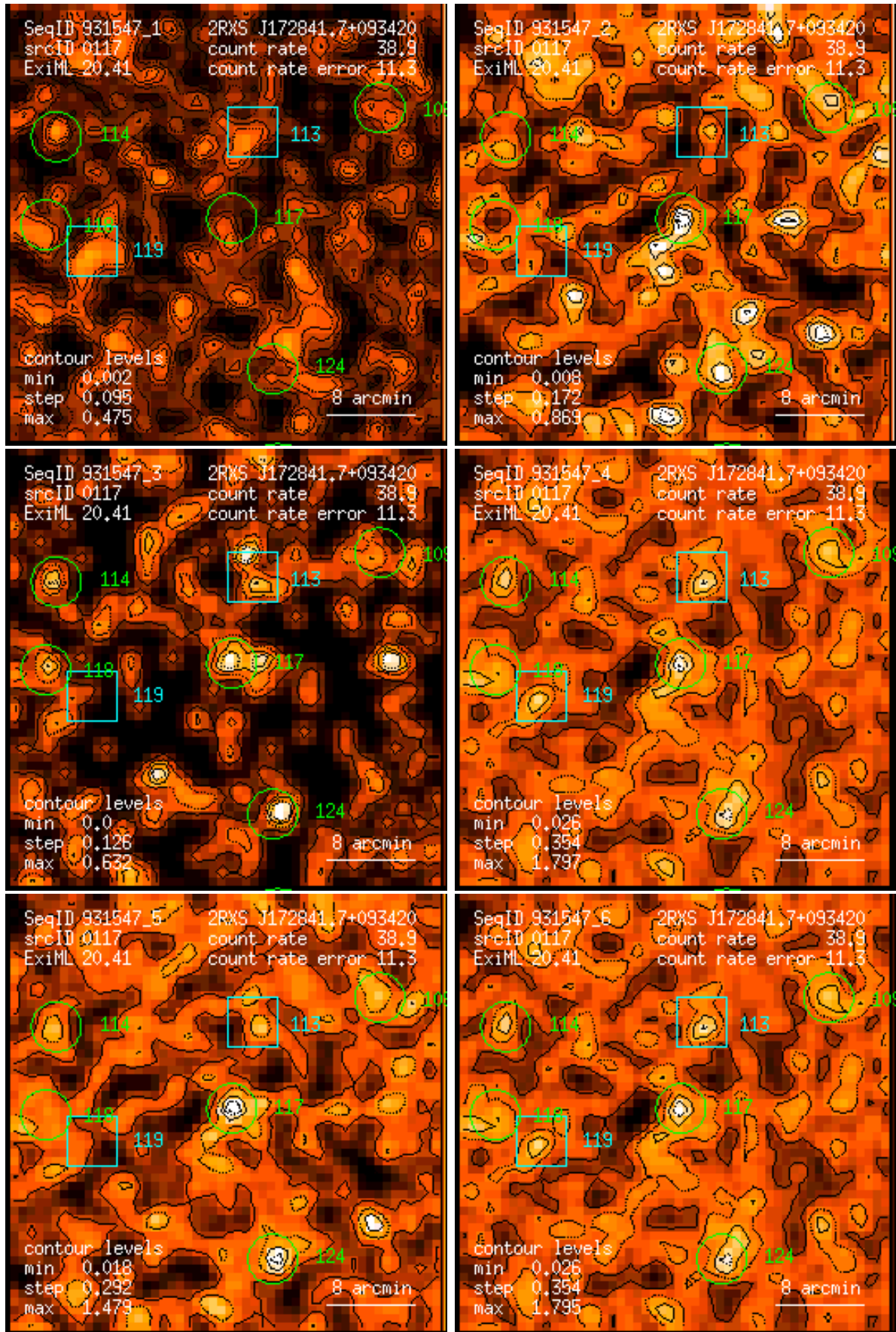
Figure 117: RASS 931547: detection 0117: band rate images, Gaussian filter: (1) PSPC channels 11 – 41, (2) 52 – 90, (3) 91 – 201, (4) 11 – 235, (5) 52 – 201, (6) 11 – 201. Broad band rates in counts/ks. Band rate contour levels in counts/ks/arcmin 2 .
