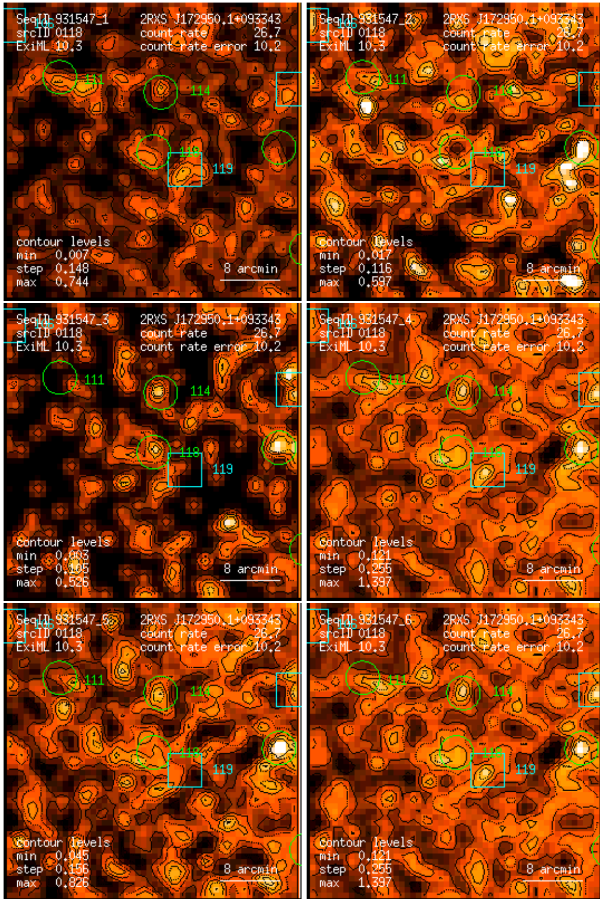
Figure 118: RASS 931547: detection 0118: band rate images, Gaussian filter: (1) PSPC channels 11 – 41, (2) 52 – 90, (3) 91 – 201, (4) 11 – 235, (5) 52 – 201, (6) 11 – 201. Broad band rates in counts/ks. Band rate contour levels in counts/ks/arcmin 2 .
