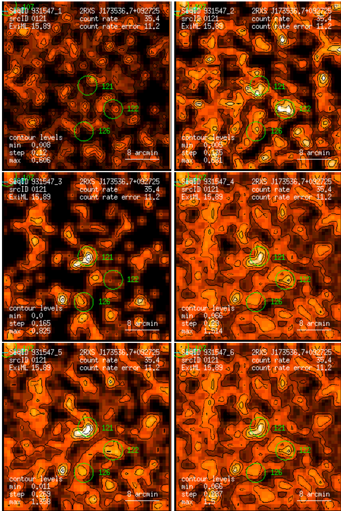
Figure 121: RASS 931547: detection 0121: band rate images, Gaussian filter: (1) PSPC channels 11 – 41, (2) 52 – 90, (3) 91 – 201, (4) 11 – 235, (5) 52 – 201, (6) 11 – 201. Broad band rates in counts/ks. Band rate contour levels in counts/ks/arcmin 2 .
