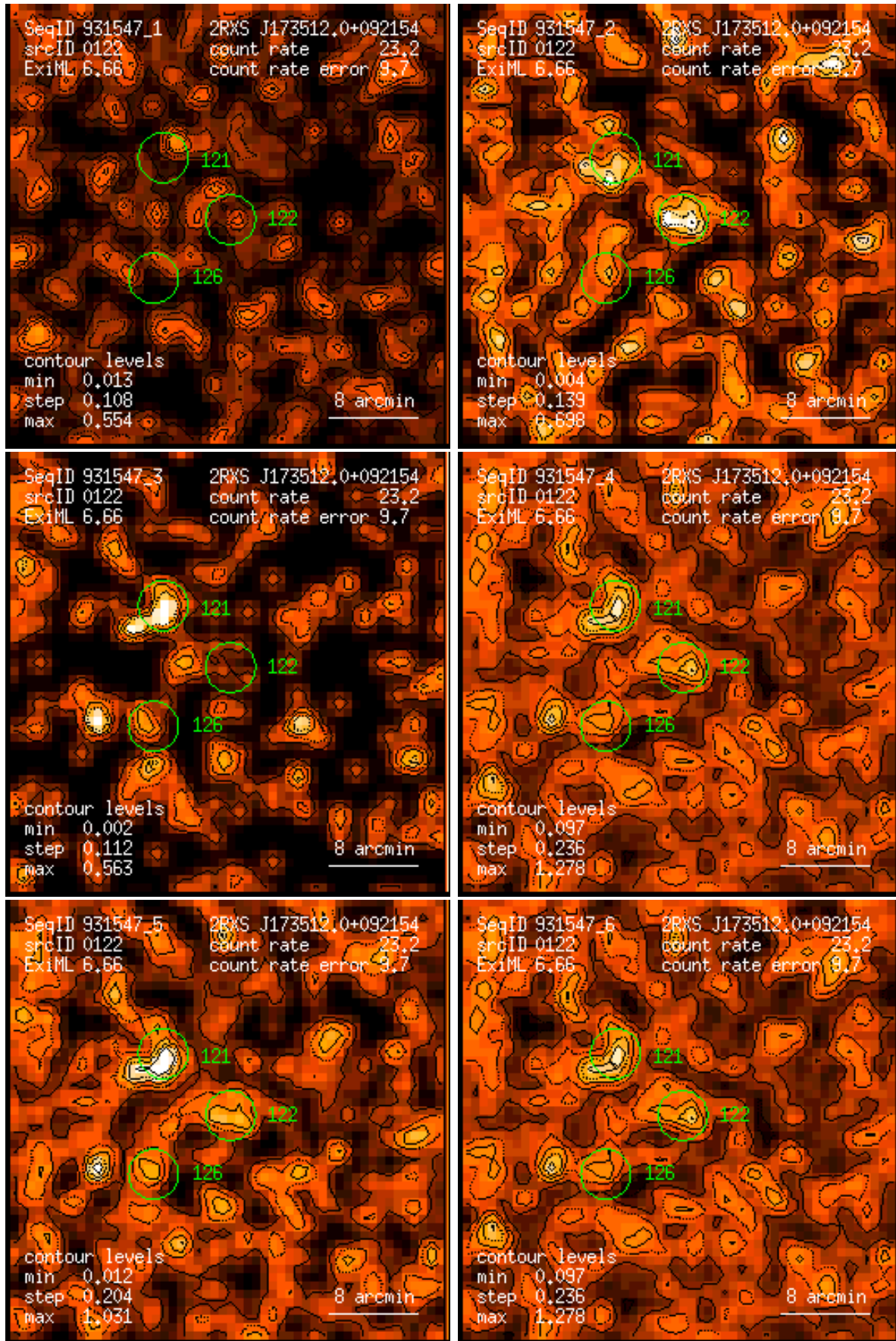
Figure 122: RASS 931547: detection 0122: band rate images, Gaussian filter: (1) PSPC channels 11 – 41, (2) 52 – 90, (3) 91 – 201, (4) 11 – 235, (5) 52 – 201, (6) 11 – 201. Broad band rates in counts/ks. Band rate contour levels in counts/ks/arcmin 2 .
