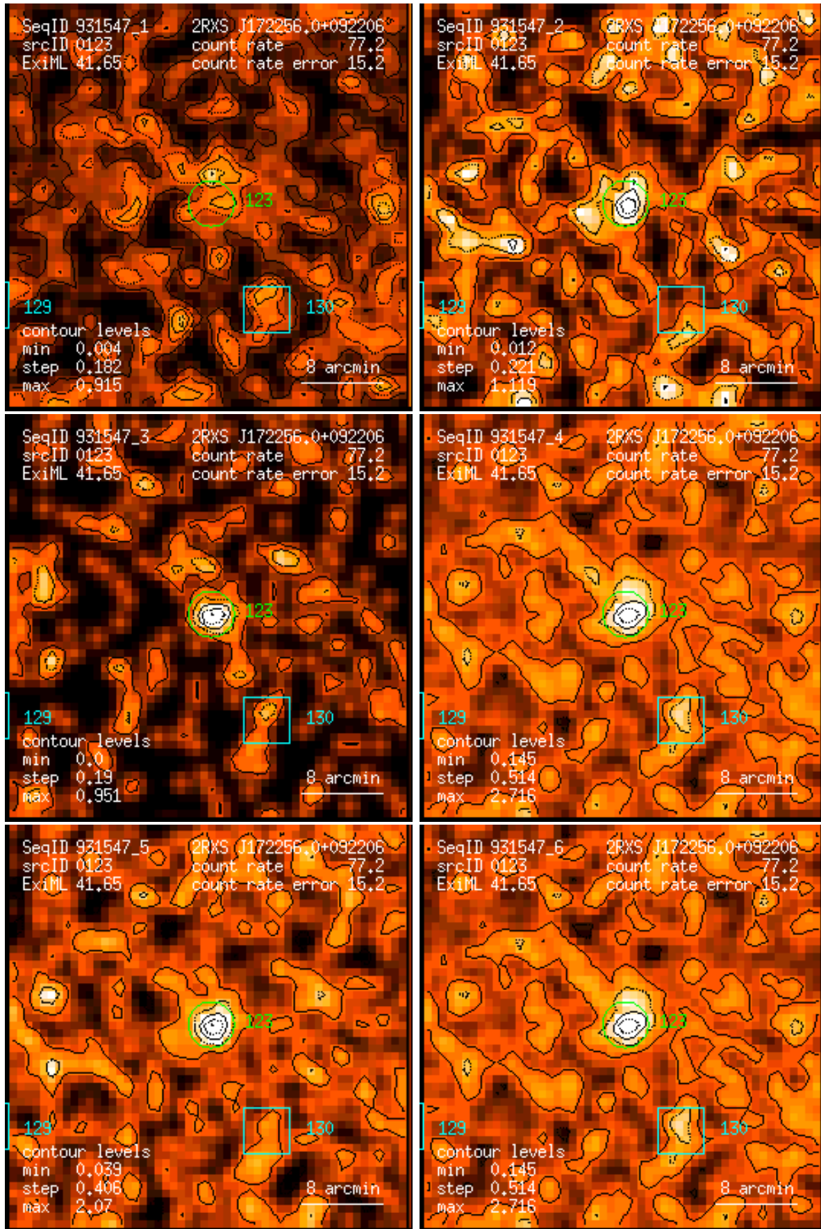
Figure 123: RASS 931547: detection 0123: band rate images, Gaussian filter: (1) PSPC channels 11 – 41, (2) 52 – 90, (3) 91 – 201, (4) 11 – 235, (5) 52 – 201, (6) 11 – 201. Broad band rates in counts/ks. Band rate contour levels in counts/ks/arcmin 2 .
