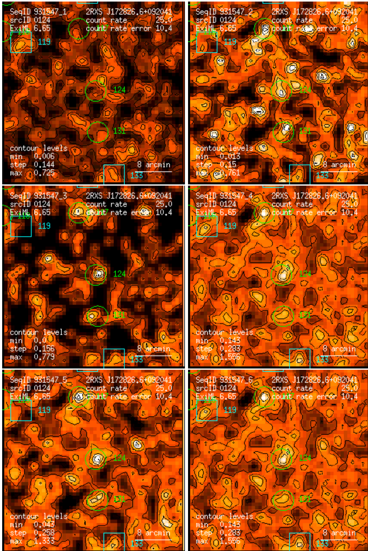
Figure 124: RASS 931547: detection 0124: band rate images, Gaussian filter: (1) PSPC channels 11 – 41, (2) 52 – 90, (3) 91 – 201, (4) 11 – 235, (5) 52 – 201, (6) 11 – 201. Broad band rates in counts/ks. Band rate contour levels in counts/ks/arcmin 2 .
