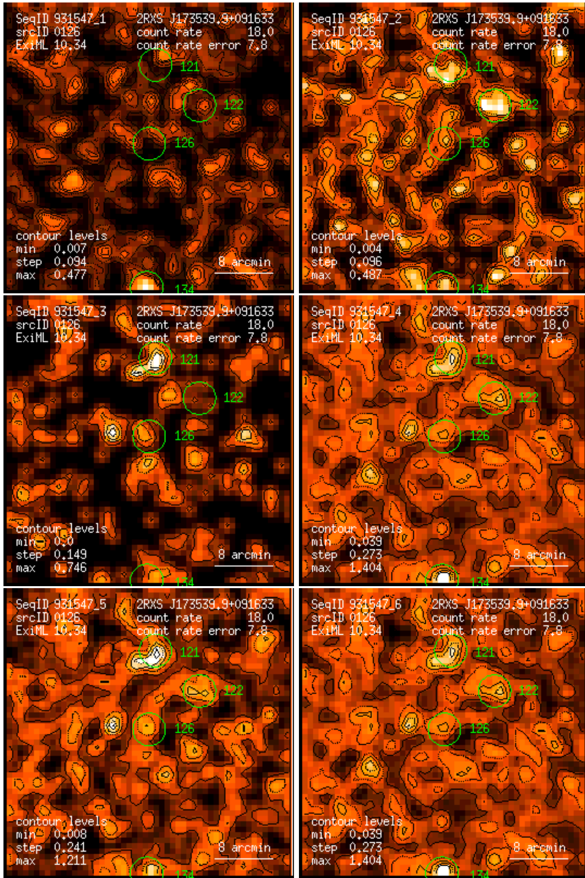
Figure 126: RASS 931547: detection 0126: band rate images, Gaussian filter: (1) PSPC channels 11 – 41, (2) 52 – 90, (3) 91 – 201, (4) 11 – 235, (5) 52 – 201, (6) 11 – 201. Broad band rates in counts/ks. Band rate contour levels in counts/ks/arcmin 2 .
