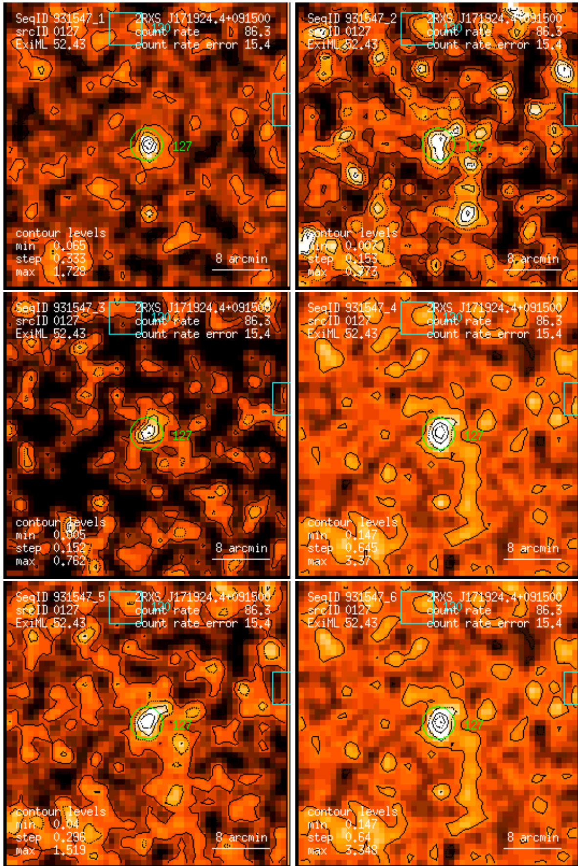
Figure 127: RASS 931547: detection 0127: band rate images, Gaussian filter: (1) PSPC channels 11 – 41, (2) 52 – 90, (3) 91 – 201, (4) 11 – 235, (5) 52 – 201, (6) 11 – 201. Broad band rates in counts/ks. Band rate contour levels in counts/ks/arcmin 2 .
