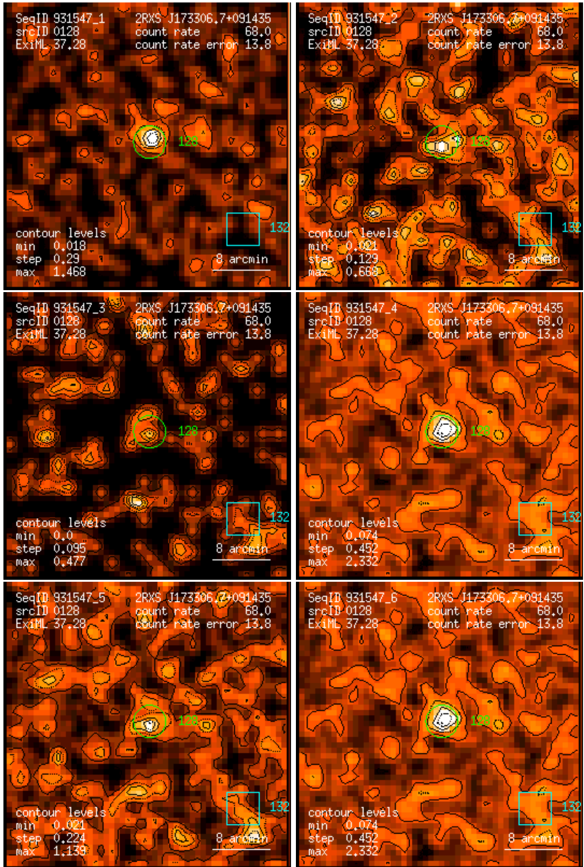
Figure 128: RASS 931547: detection 0128: band rate images, Gaussian filter: (1) PSPC channels 11 – 41, (2) 52 – 90, (3) 91 – 201, (4) 11 – 235, (5) 52 – 201, (6) 11 – 201. Broad band rates in counts/ks. Band rate contour levels in counts/ks/arcmin 2 .
