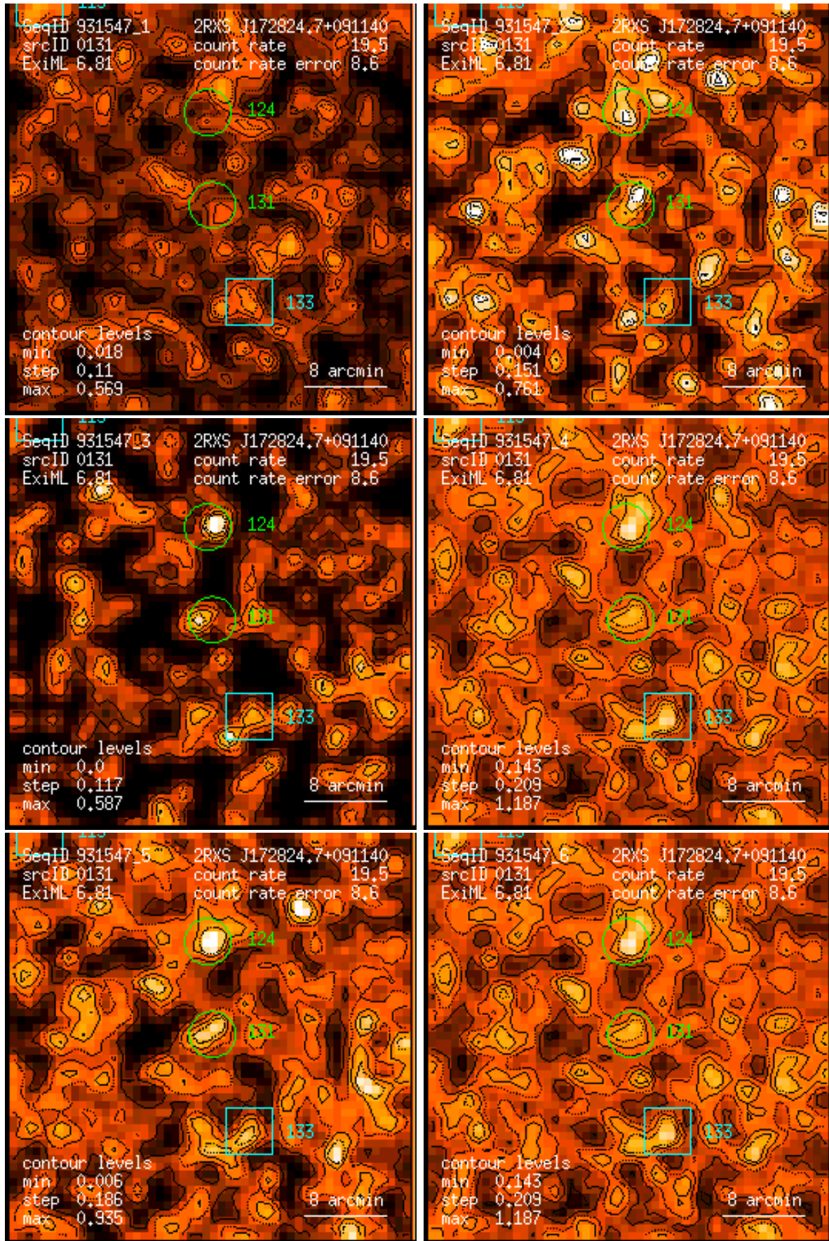
Figure 131: RASS 931547: detection 0131: band rate images, Gaussian filter: (1) PSPC channels 11 – 41, (2) 52 – 90, (3) 91 – 201, (4) 11 – 235, (5) 52 – 201, (6) 11 – 201. Broad band rates in counts/ks. Band rate contour levels in counts/ks/arcmin 2 .
