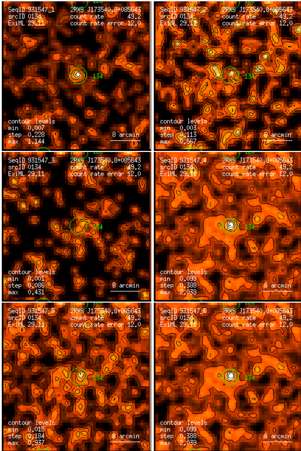
Figure 134: RASS 931547: detection 0134: band rate images, Gaussian filter: (1) PSPC channels 11 – 41, (2) 52 – 90, (3) 91 – 201, (4) 11 – 235, (5) 52 – 201, (6) 11 – 201. Broad band rates in counts/ks. Band rate contour levels in counts/ks/arcmin 2 .
