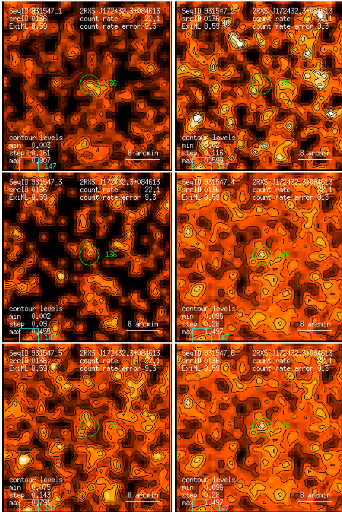
Figure 136: RASS 931547: detection 0136: band rate images, Gaussian filter: (1) PSPC channels 11 – 41, (2) 52 – 90, (3) 91 – 201, (4) 11 – 235, (5) 52 – 201, (6) 11 – 201. Broad band rates in counts/ks. Band rate contour levels in counts/ks/arcmin 2 .
