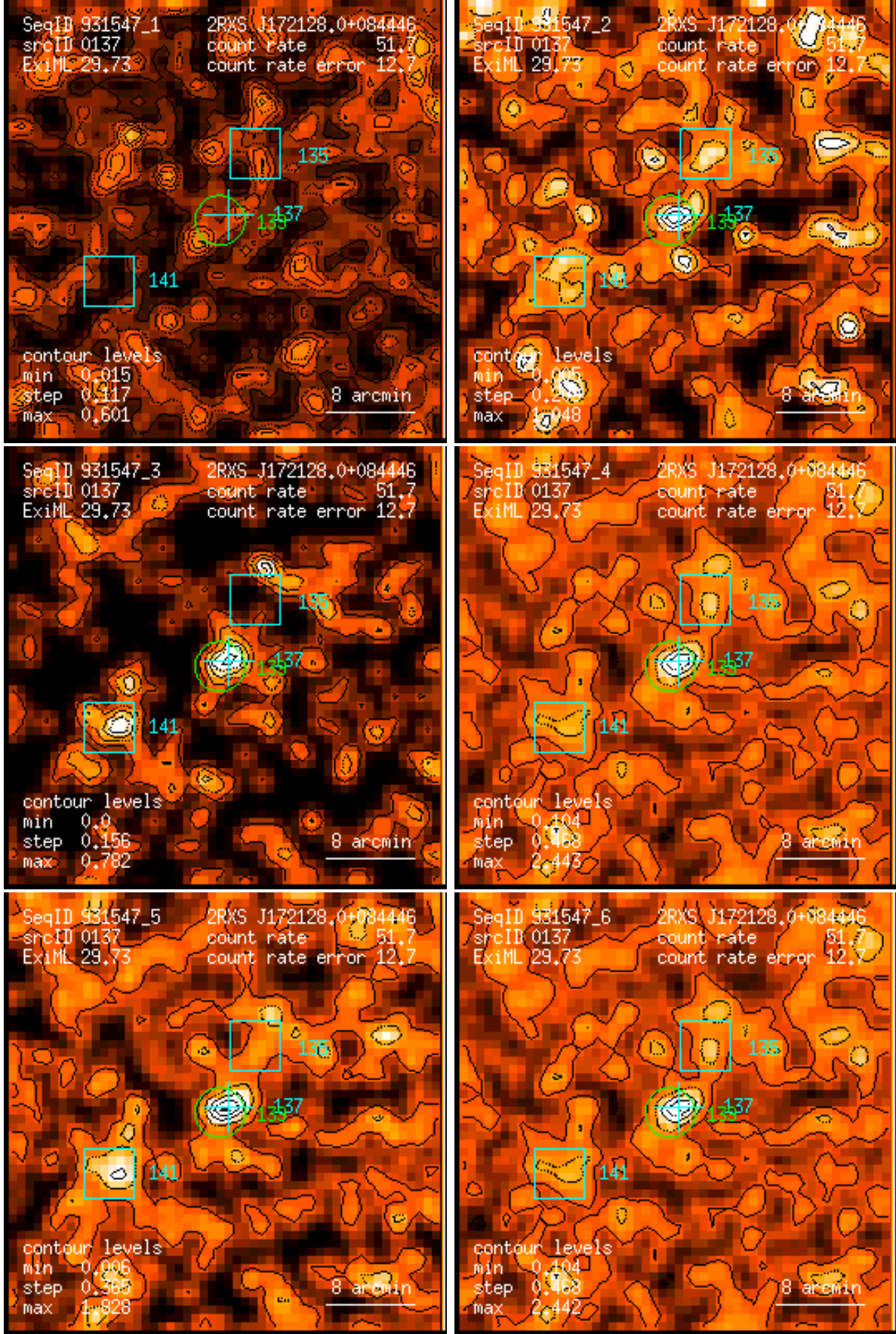
Figure 137: RASS 931547: detection 0137: band rate images, Gaussian filter: (1) PSPC channels 11 – 41, (2) 52 – 90, (3) 91 – 201, (4) 11 – 235, (5) 52 – 201, (6) 11 – 201. Broad band rates in counts/ks. Band rate contour levels in counts/ks/arcmin 2 .
