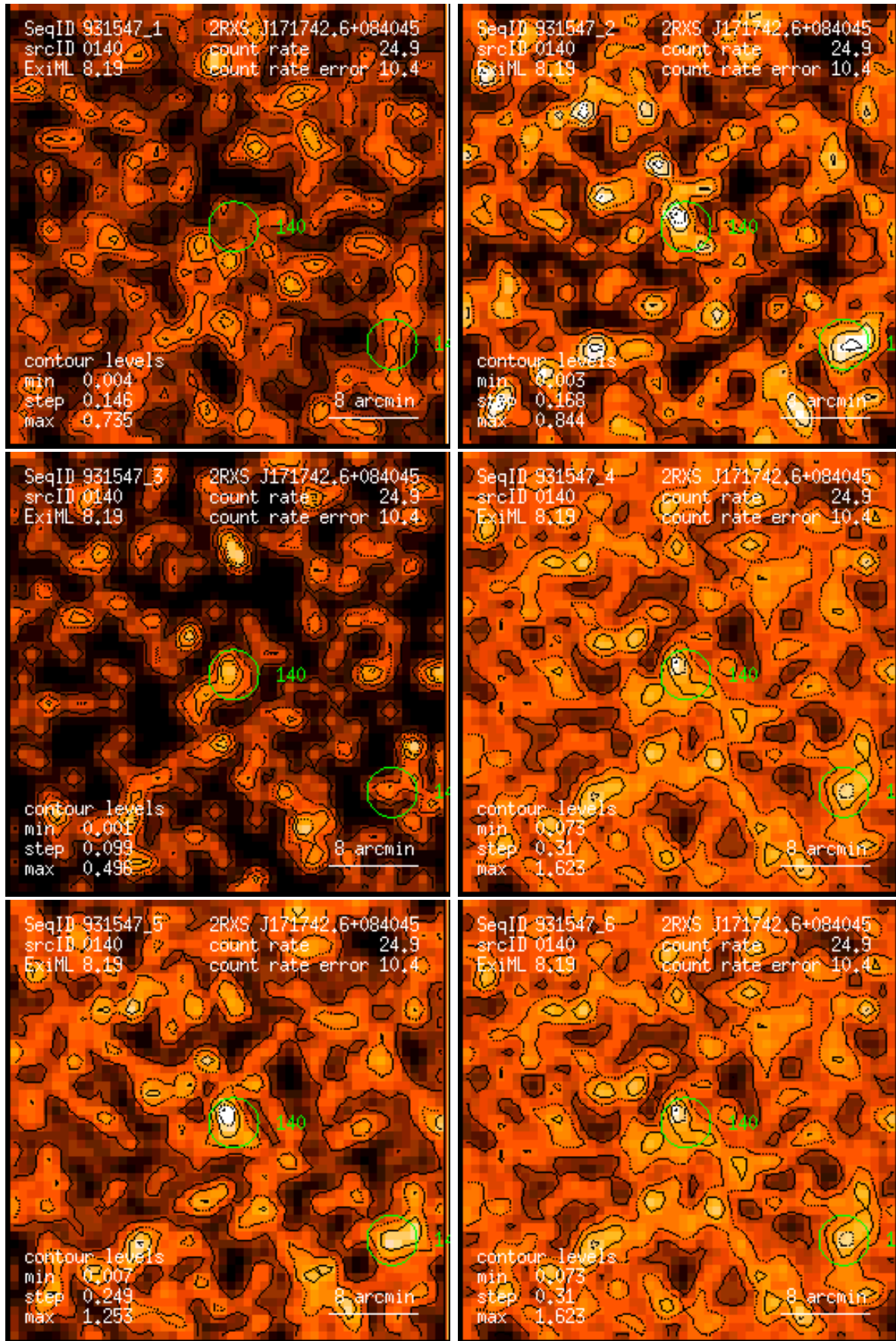
Figure 140: RASS 931547: detection 0140: band rate images, Gaussian filter: (1) PSPC channels 11 – 41, (2) 52 – 90, (3) 91 – 201, (4) 11 – 235, (5) 52 – 201, (6) 11 – 201. Broad band rates in counts/ks. Band rate contour levels in counts/ks/arcmin 2 .
