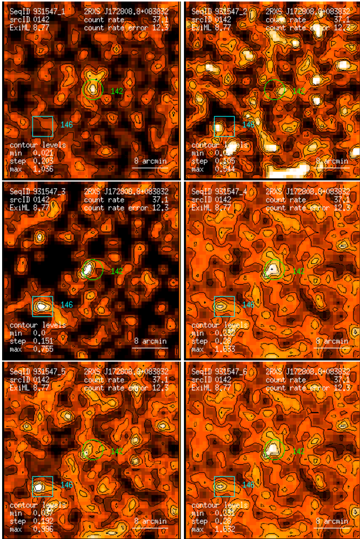
Figure 142: RASS 931547: detection 0142: band rate images, Gaussian filter: (1) PSPC channels 11 – 41, (2) 52 – 90, (3) 91 – 201, (4) 11 – 235, (5) 52 – 201, (6) 11 – 201. Broad band rates in counts/ks. Band rate contour levels in counts/ks/arcmin 2 .
