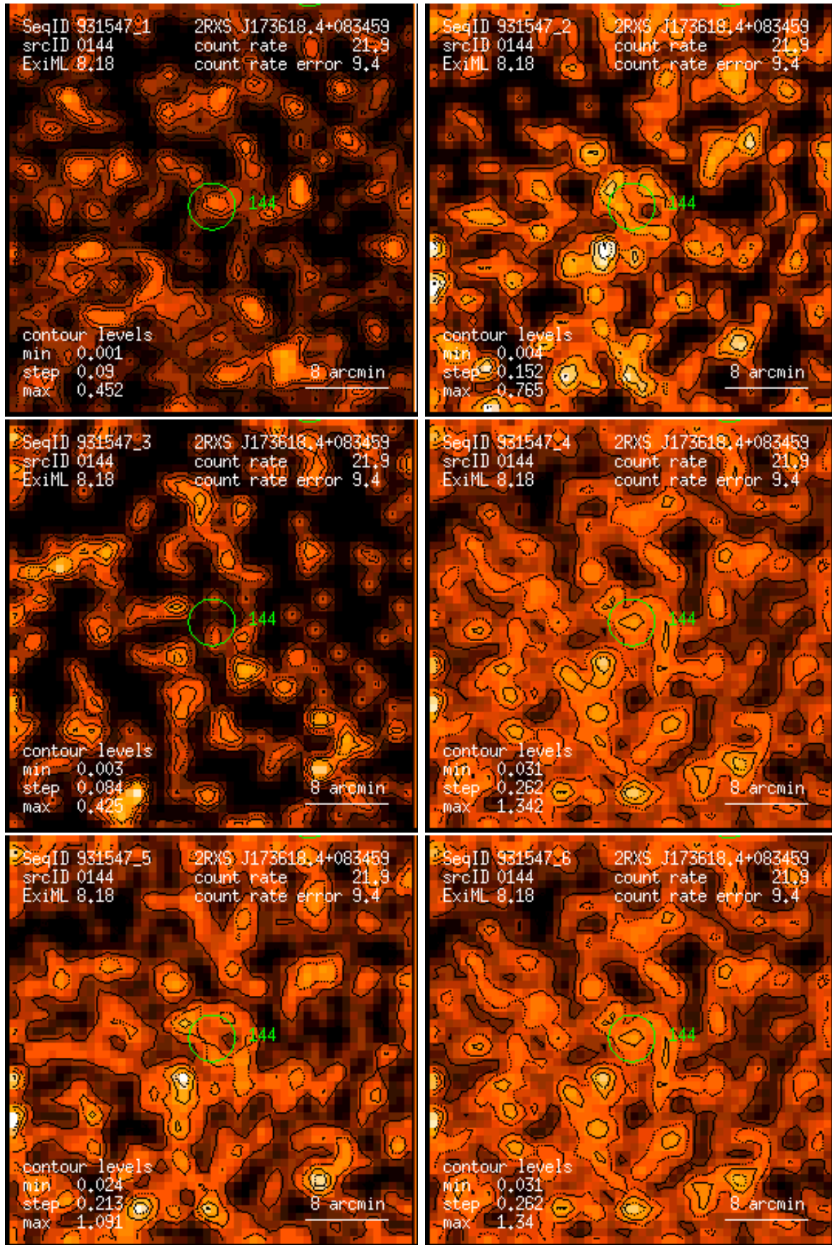
Figure 144: RASS 931547: detection 0144: band rate images, Gaussian filter: (1) PSPC channels 11 – 41, (2) 52 – 90, (3) 91 – 201, (4) 11 – 235, (5) 52 – 201, (6) 11 – 201. Broad band rates in counts/ks. Band rate contour levels in counts/ks/arcmin 2 .
