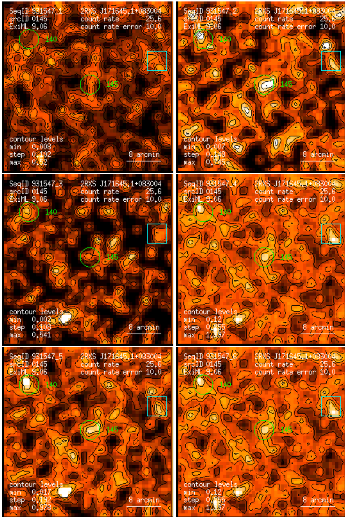
Figure 145: RASS 931547: detection 0145: band rate images, Gaussian filter: (1) PSPC channels 11 – 41, (2) 52 – 90, (3) 91 – 201, (4) 11 – 235, (5) 52 – 201, (6) 11 – 201. Broad band rates in counts/ks. Band rate contour levels in counts/ks/arcmin 2 .
