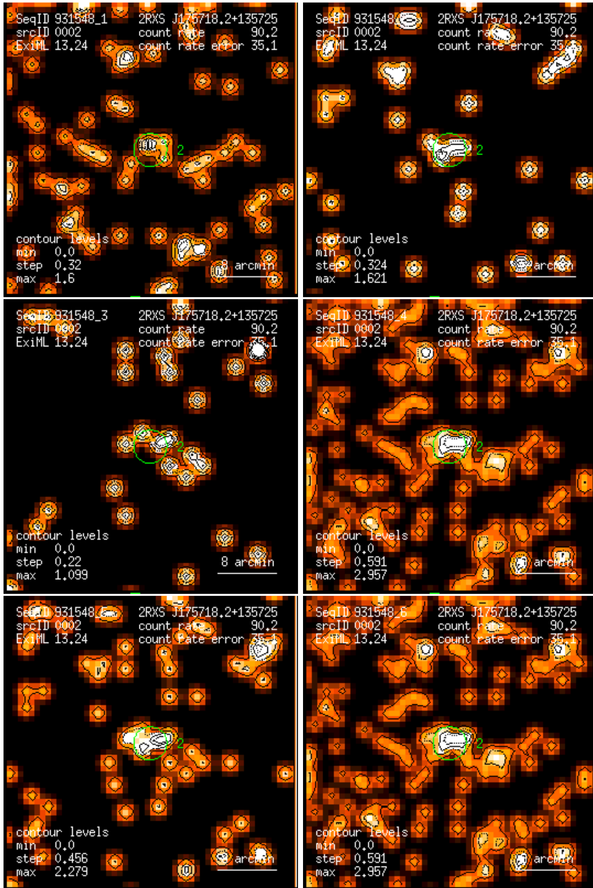
Figure 2: RASS 931548: detection 0002: band rate images, Gaussian filter: (1) PSPC channels 11 – 41, (2) 52 – 90, (3) 91 – 201, (4) 11 – 235, (5) 52 – 201, (6) 11 – 201. Broad band rates in counts/ks. Band rate contour levels in counts/ks/arcmin 2 .
