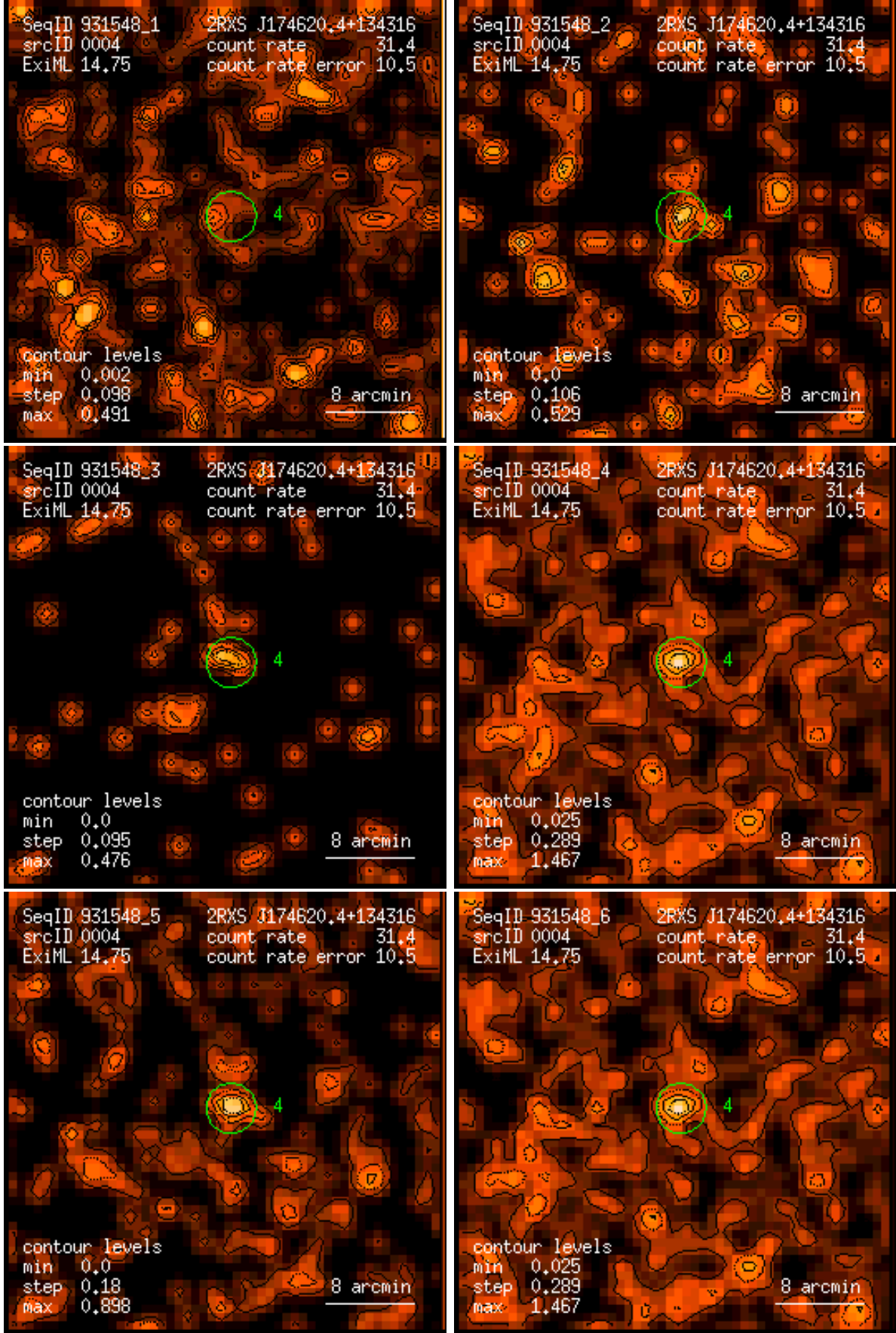
Figure 4: RASS 931548: detection 0004: band rate images, Gaussian filter: (1) PSPC channels 11 – 41, (2) 52 – 90, (3) 91 – 201, (4) 11 – 235, (5) 52 – 201, (6) 11 – 201. Broad band rates in counts/ks. Band rate contour levels in counts/ks/arcmin 2 .
