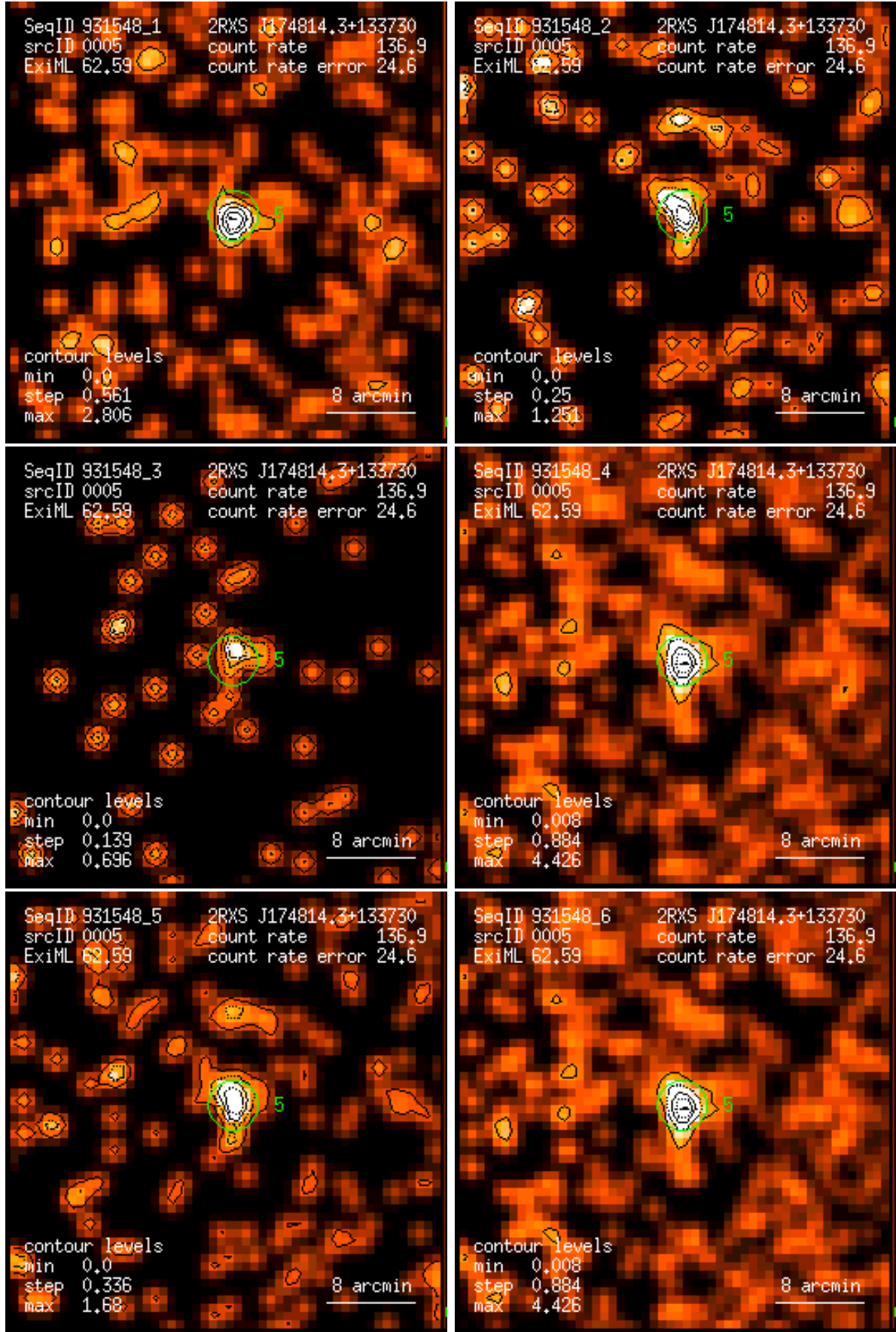
Figure 5: RASS 931548: detection 0005: band rate images, Gaussian filter: (1) PSPC channels 11 – 41, (2) 52 – 90, (3) 91 – 201, (4) 11 – 235, (5) 52 – 201, (6) 11 – 201. Broad band rates in counts/ks. Band rate contour levels in counts/ks/arcmin 2 .
