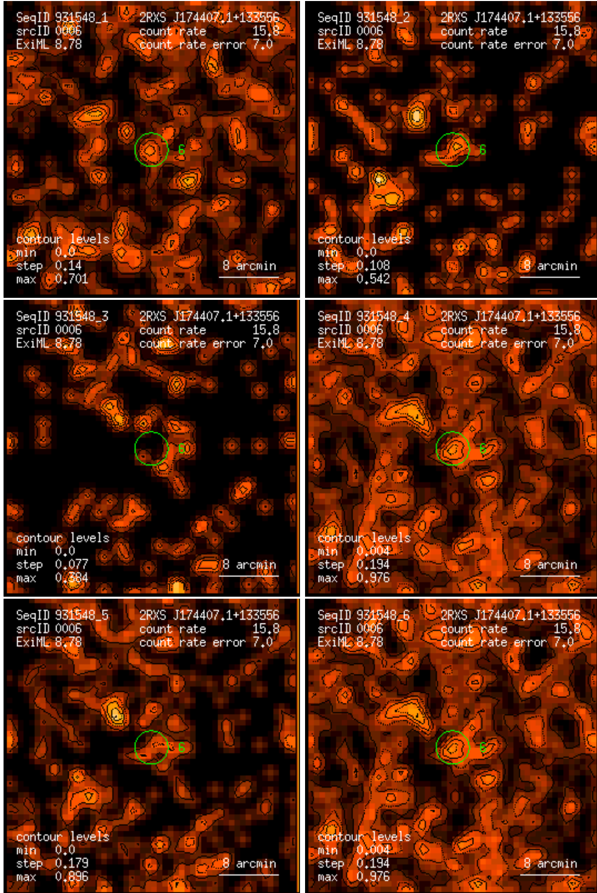
Figure 6: RASS 931548: detection 0006: band rate images, Gaussian filter: (1) PSPC channels 11 – 41, (2) 52 – 90, (3) 91 – 201, (4) 11 – 235, (5) 52 – 201, (6) 11 – 201. Broad band rates in counts/ks. Band rate contour levels in counts/ks/arcmin 2 .
