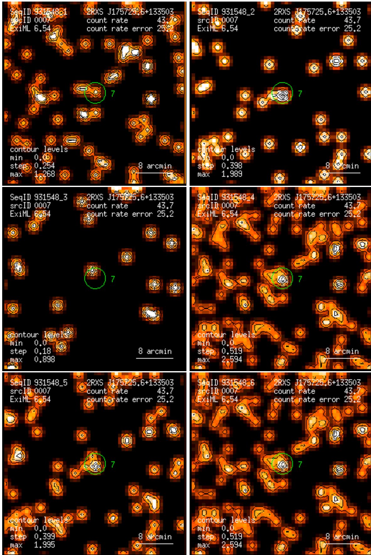
Figure 7: RASS 931548: detection 0007: band rate images, Gaussian filter: (1) PSPC channels 11 – 41, (2) 52 – 90, (3) 91 – 201, (4) 11 – 235, (5) 52 – 201, (6) 11 – 201. Broad band rates in counts/ks. Band rate contour levels in counts/ks/arcmin 2 .
