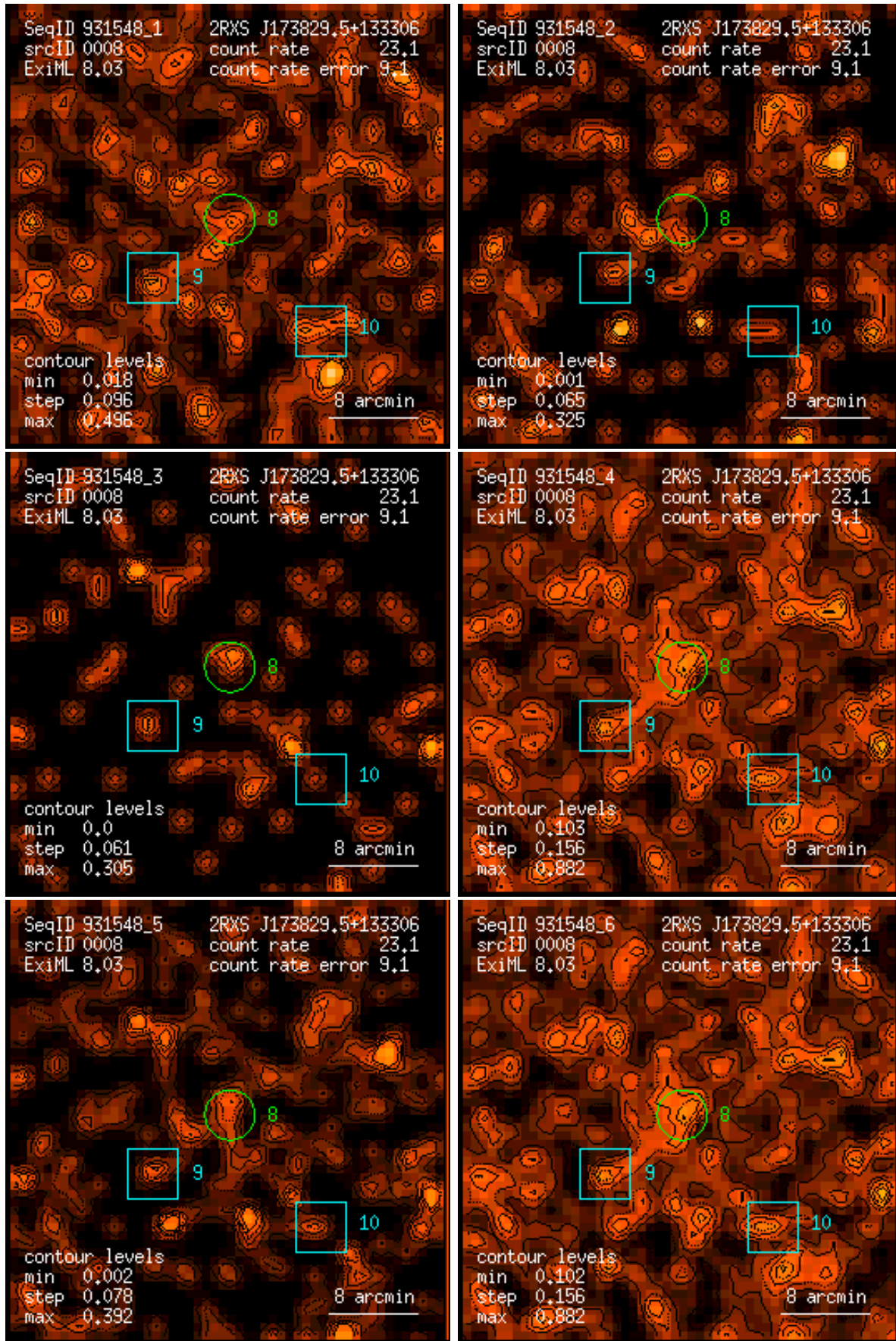
Figure 8: RASS 931548: detection 0008: band rate images, Gaussian filter: (1) PSPC channels 11 – 41, (2) 52 – 90, (3) 91 – 201, (4) 11 – 235, (5) 52 – 201, (6) 11 – 201. Broad band rates in counts/ks. Band rate contour levels in counts/ks/arcmin 2 .
