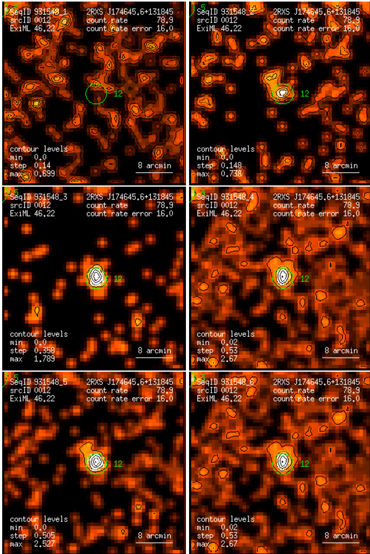
Figure 12: RASS 931548: detection 0012: band rate images, Gaussian filter: (1) PSPC channels 11 – 41, (2) 52 – 90, (3) 91 – 201, (4) 11 – 235, (5) 52 – 201, (6) 11 – 201. Broad band rates in counts/ks. Band rate contour levels in counts/ks/arcmin 2 .
