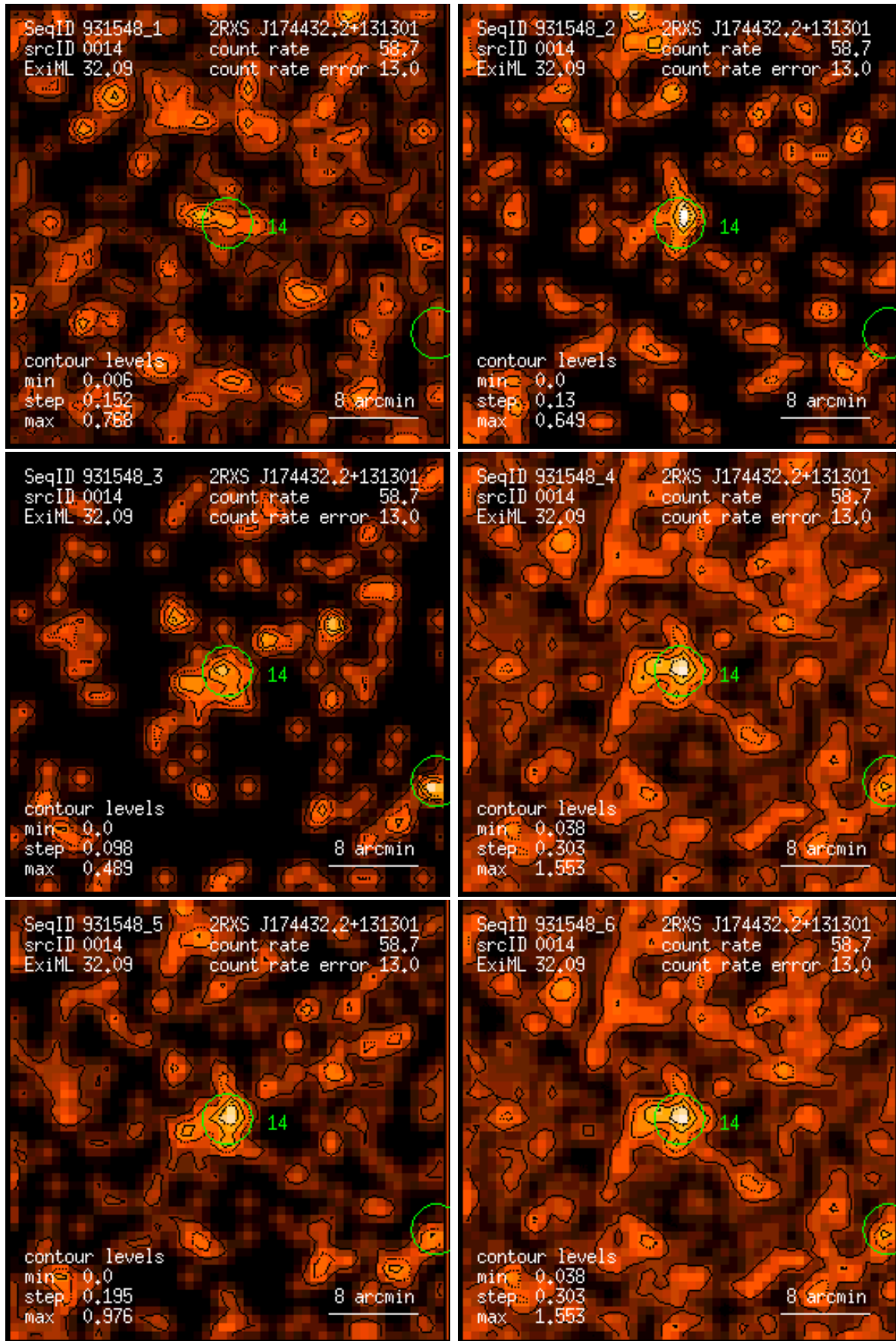
Figure 14: RASS 931548: detection 0014: band rate images, Gaussian filter: (1) PSPC channels 11 – 41, (2) 52 – 90, (3) 91 – 201, (4) 11 – 235, (5) 52 – 201, (6) 11 – 201. Broad band rates in counts/ks. Band rate contour levels in counts/ks/arcmin 2 .
