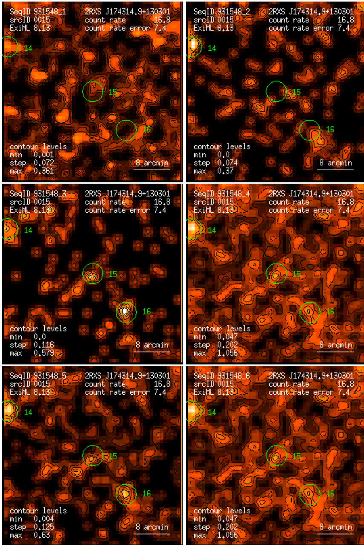
Figure 15: RASS 931548: detection 0015: band rate images, Gaussian filter: (1) PSPC channels 11 – 41, (2) 52 – 90, (3) 91 – 201, (4) 11 – 235, (5) 52 – 201, (6) 11 – 201. Broad band rates in counts/ks. Band rate contour levels in counts/ks/arcmin 2 .
