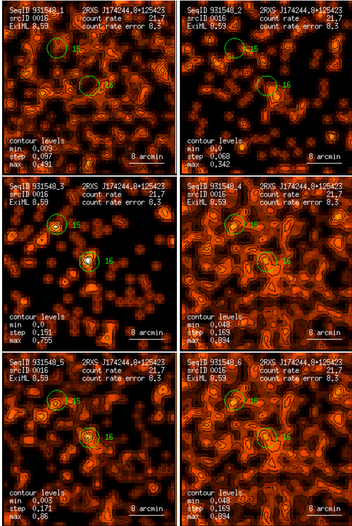
Figure 16: RASS 931548: detection 0016: band rate images, Gaussian filter: (1) PSPC channels 11 – 41, (2) 52 – 90, (3) 91 – 201, (4) 11 – 235, (5) 52 – 201, (6) 11 – 201. Broad band rates in counts/ks. Band rate contour levels in counts/ks/arcmin 2 .
