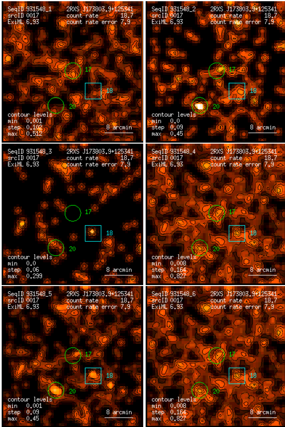
Figure 17: RASS 931548: detection 0017: band rate images, Gaussian filter: (1) PSPC channels 11 – 41, (2) 52 – 90, (3) 91 – 201, (4) 11 – 235, (5) 52 – 201, (6) 11 – 201. Broad band rates in counts/ks. Band rate contour levels in counts/ks/arcmin 2 .
