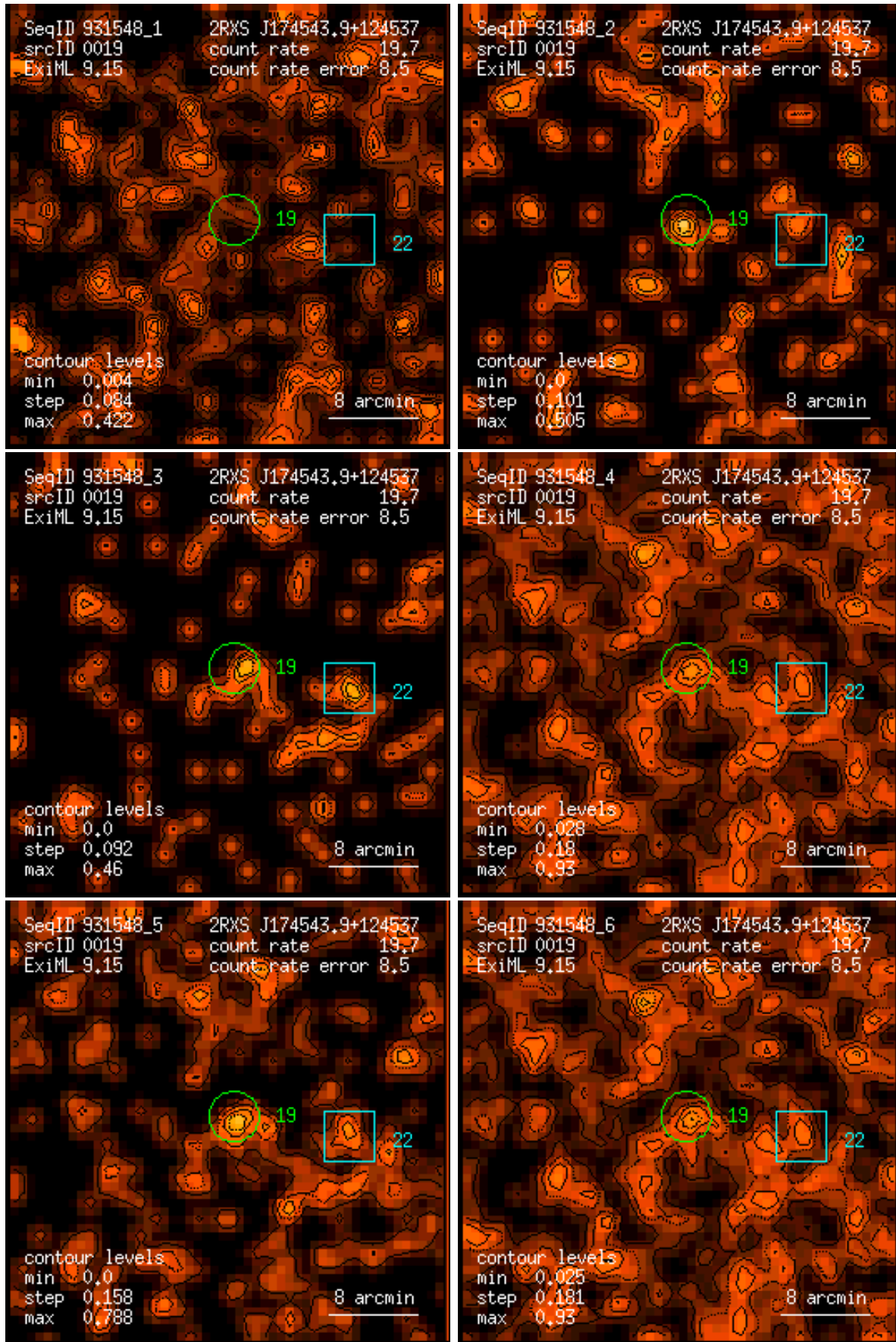
Figure 19: RASS 931548: detection 0019: band rate images, Gaussian filter: (1) PSPC channels 11 – 41, (2) 52 – 90, (3) 91 – 201, (4) 11 – 235, (5) 52 – 201, (6) 11 – 201. Broad band rates in counts/ks. Band rate contour levels in counts/ks/arcmin 2 .
