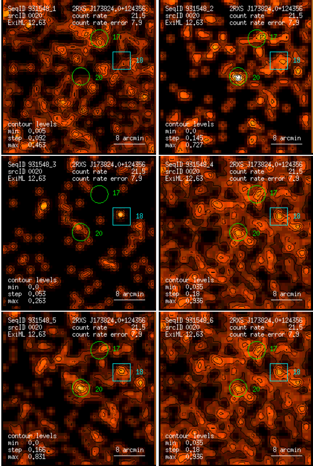
Figure 20: RASS 931548: detection 0020: band rate images, Gaussian filter: (1) PSPC channels 11 – 41, (2) 52 – 90, (3) 91 – 201, (4) 11 – 235, (5) 52 – 201, (6) 11 – 201. Broad band rates in counts/ks. Band rate contour levels in counts/ks/arcmin 2 .
