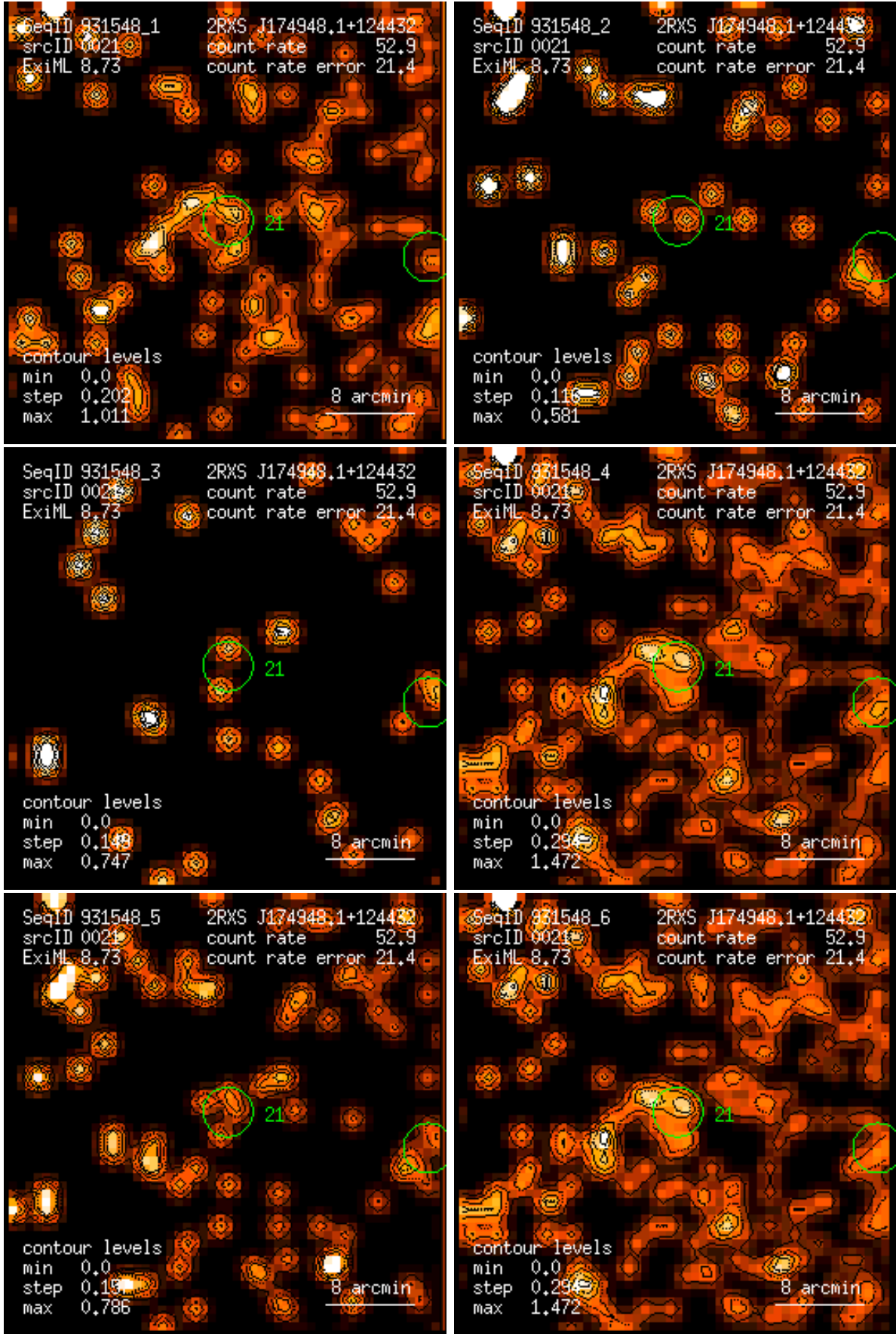
Figure 21: RASS 931548: detection 0021: band rate images, Gaussian filter: (1) PSPC channels 11 – 41, (2) 52 – 90, (3) 91 – 201, (4) 11 – 235, (5) 52 – 201, (6) 11 – 201. Broad band rates in counts/ks. Band rate contour levels in counts/ks/arcmin 2 .
