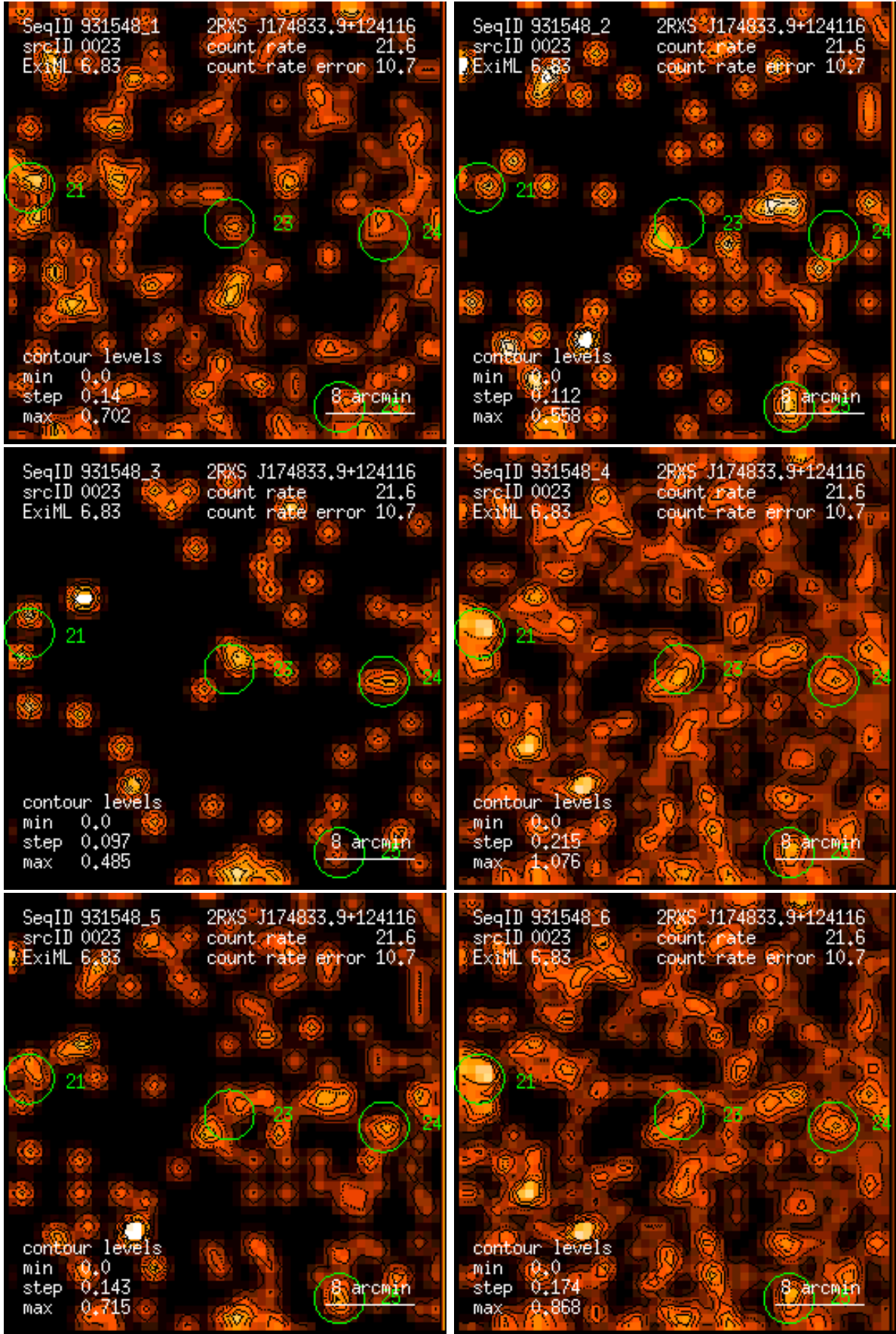
Figure 23: RASS 931548: detection 0023: band rate images, Gaussian filter: (1) PSPC channels 11 – 41, (2) 52 – 90, (3) 91 – 201, (4) 11 – 235, (5) 52 – 201, (6) 11 – 201. Broad band rates in counts/ks. Band rate contour levels in counts/ks/arcmin 2 .
