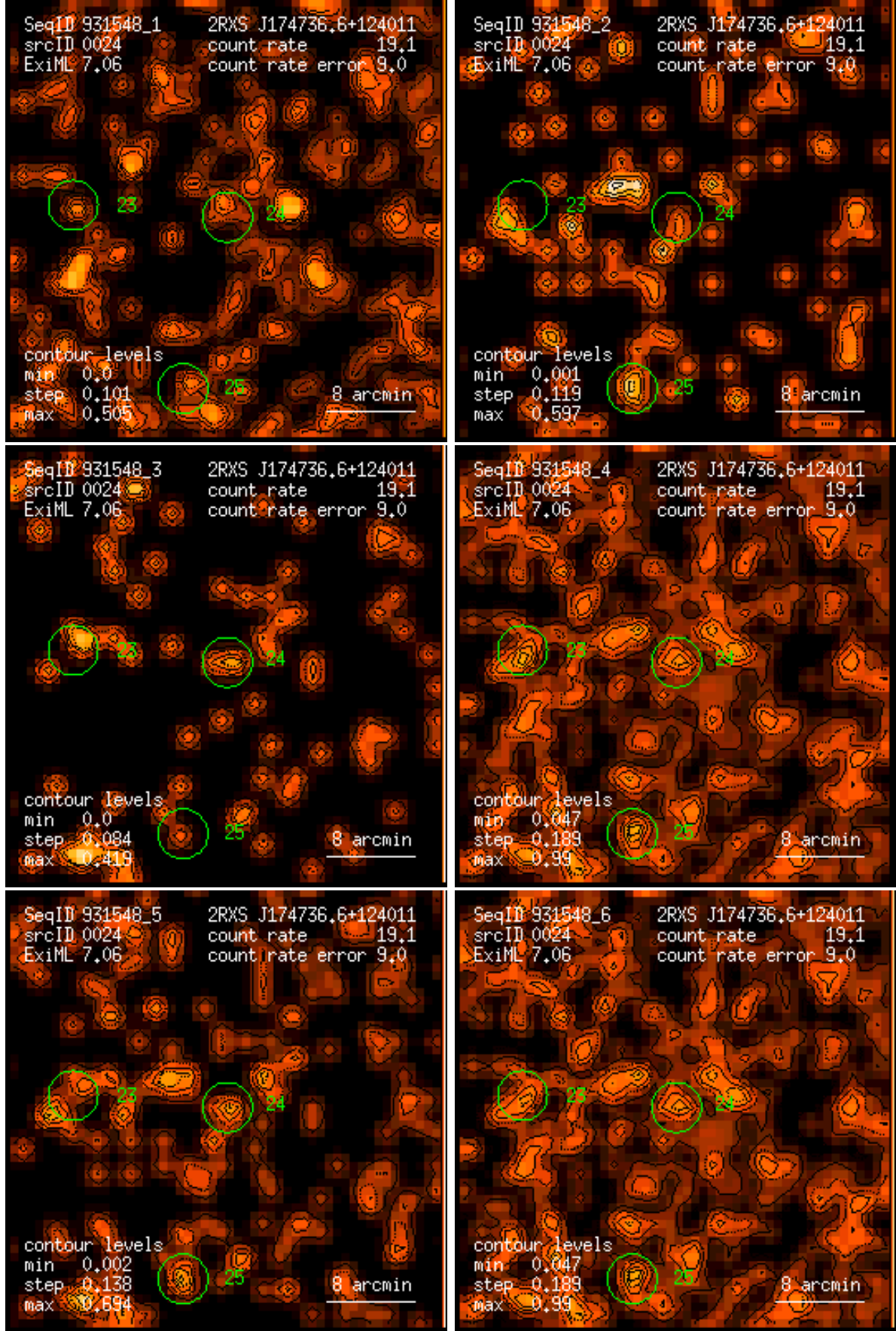
Figure 24: RASS 931548: detection 0024: band rate images, Gaussian filter: (1) PSPC channels 11 – 41, (2) 52 – 90, (3) 91 – 201, (4) 11 – 235, (5) 52 – 201, (6) 11 – 201. Broad band rates in counts/ks. Band rate contour levels in counts/ks/arcmin 2 .
