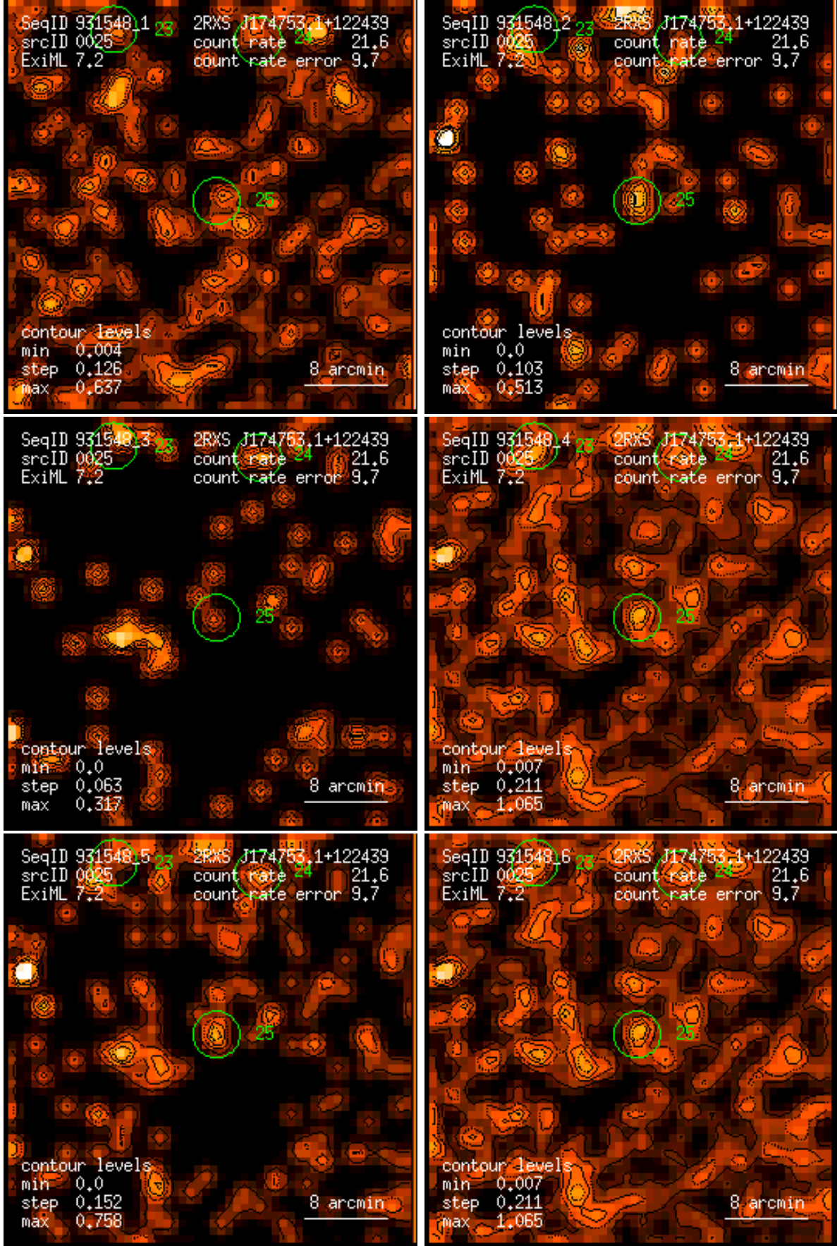
Figure 25: RASS 931548: detection 0025: band rate images, Gaussian filter: (1) PSPC channels 11 – 41, (2) 52 – 90, (3) 91 – 201, (4) 11 – 235, (5) 52 – 201, (6) 11 – 201. Broad band rates in counts/ks. Band rate contour levels in counts/ks/arcmin 2 .
