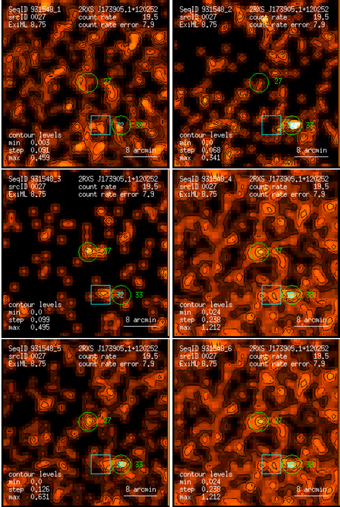
Figure 27: RASS 931548: detection 0027: band rate images, Gaussian filter: (1) PSPC channels 11 – 41, (2) 52 – 90, (3) 91 – 201, (4) 11 – 235, (5) 52 – 201, (6) 11 – 201. Broad band rates in counts/ks. Band rate contour levels in counts/ks/arcmin 2 .
