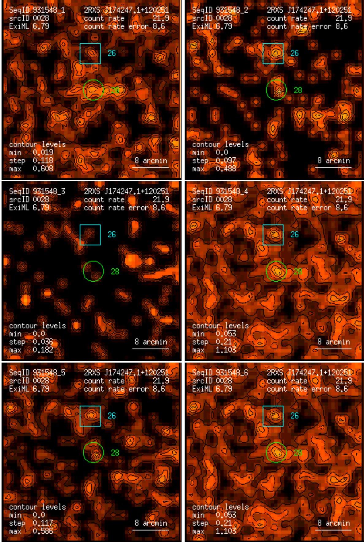
Figure 28: RASS 931548: detection 0028: band rate images, Gaussian filter: (1) PSPC channels 11 – 41, (2) 52 – 90, (3) 91 – 201, (4) 11 – 235, (5) 52 – 201, (6) 11 – 201. Broad band rates in counts/ks. Band rate contour levels in counts/ks/arcmin 2 .
