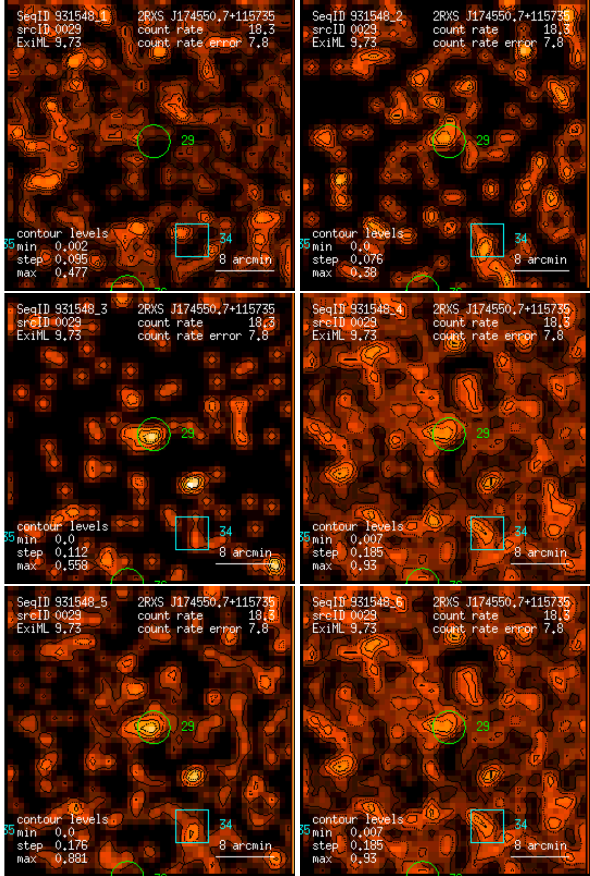
Figure 29: RASS 931548: detection 0029: band rate images, Gaussian filter: (1) PSPC channels 11 – 41, (2) 52 – 90, (3) 91 – 201, (4) 11 – 235, (5) 52 – 201, (6) 11 – 201. Broad band rates in counts/ks. Band rate contour levels in counts/ks/arcmin 2 .
