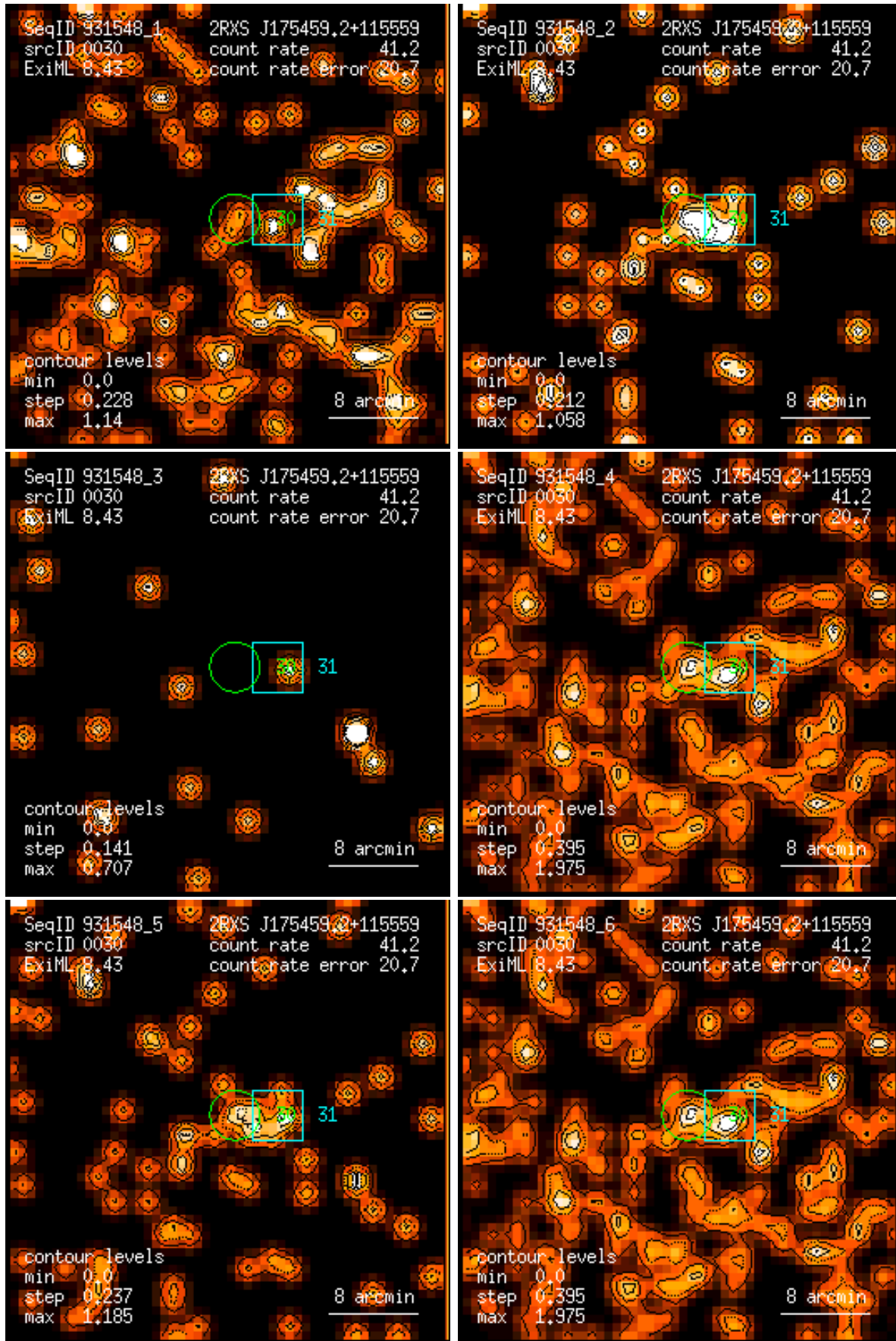
Figure 30: RASS 931548: detection 0030: band rate images, Gaussian filter: (1) PSPC channels 11 – 41, (2) 52 – 90, (3) 91 – 201, (4) 11 – 235, (5) 52 – 201, (6) 11 – 201. Broad band rates in counts/ks. Band rate contour levels in counts/ks/arcmin 2 .
