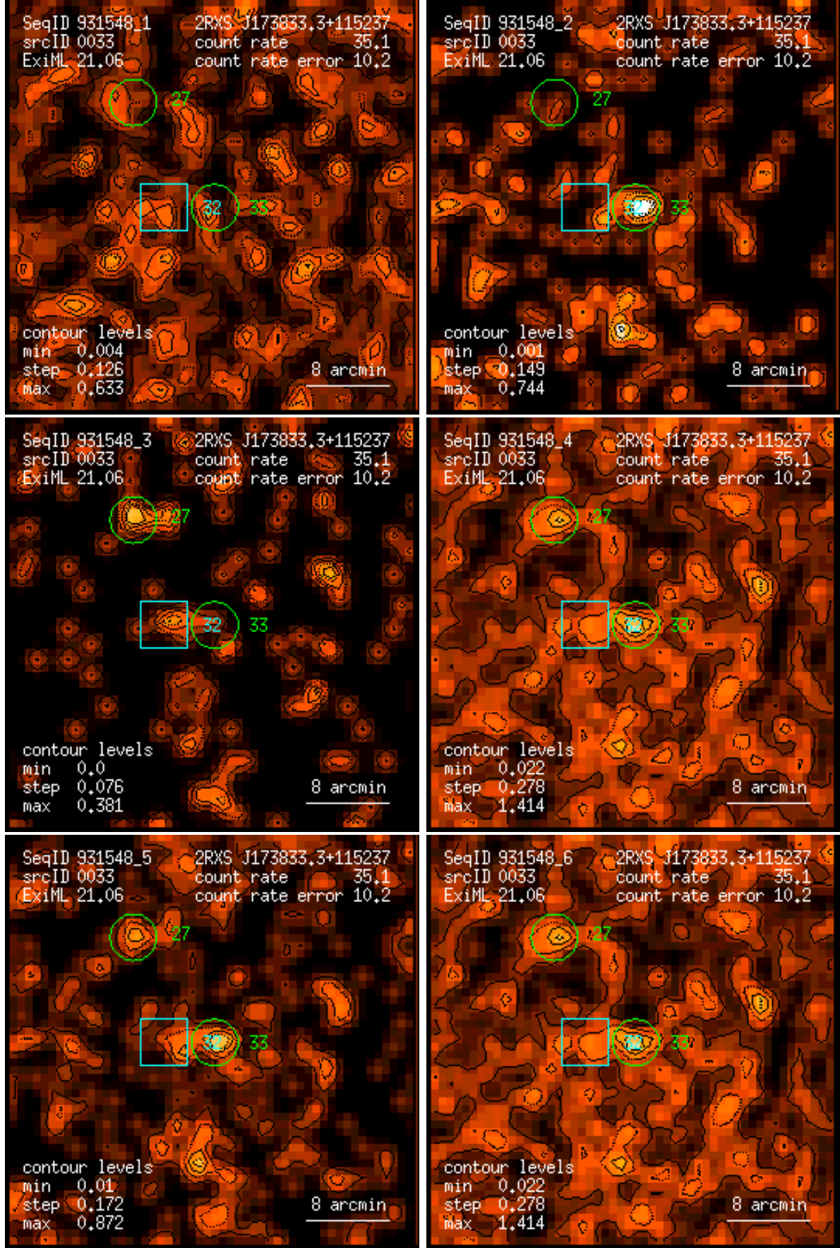
Figure 33: RASS 931548: detection 0033: band rate images, Gaussian filter: (1) PSPC channels 11 – 41, (2) 52 – 90, (3) 91 – 201, (4) 11 – 235, (5) 52 – 201, (6) 11 – 201. Broad band rates in counts/ks. Band rate contour levels in counts/ks/arcmin 2 .
