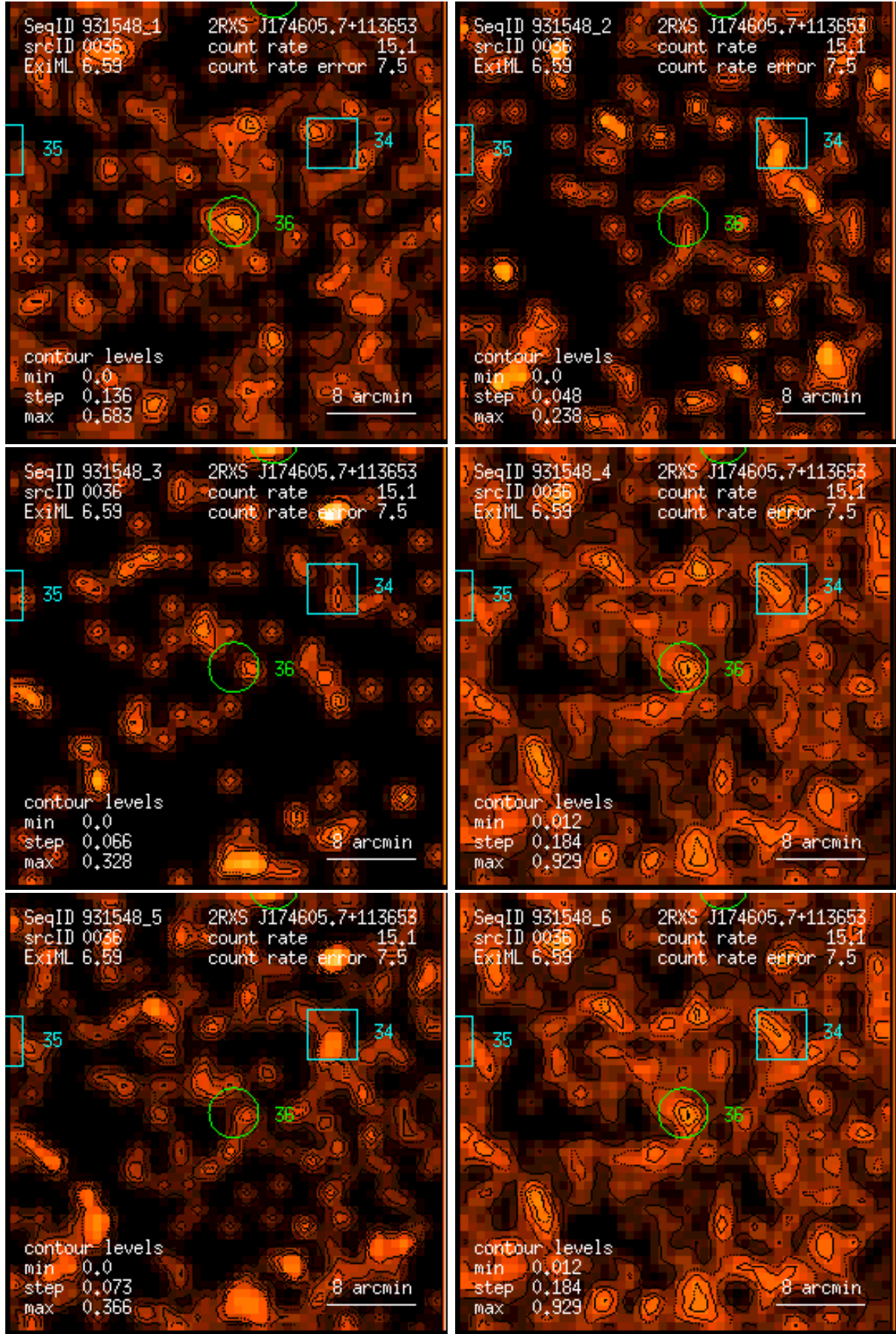
Figure 36: RASS 931548: detection 0036: band rate images, Gaussian filter: (1) PSPC channels 11 – 41, (2) 52 – 90, (3) 91 – 201, (4) 11 – 235, (5) 52 – 201, (6) 11 – 201. Broad band rates in counts/ks. Band rate contour levels in counts/ks/arcmin 2 .
