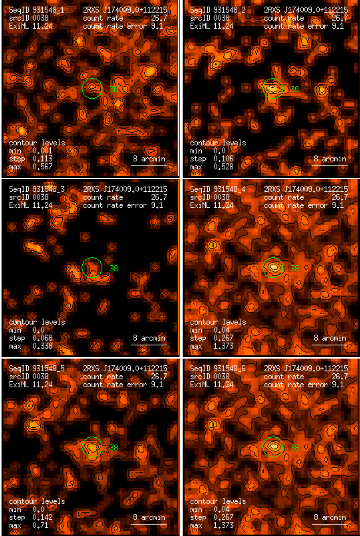
Figure 38: RASS 931548: detection 0038: band rate images, Gaussian filter: (1) PSPC channels 11 – 41, (2) 52 – 90, (3) 91 – 201, (4) 11 – 235, (5) 52 – 201, (6) 11 – 201. Broad band rates in counts/ks. Band rate contour levels in counts/ks/arcmin 2 .
