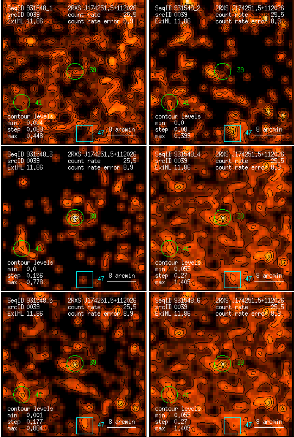
Figure 39: RASS 931548: detection 0039: band rate images, Gaussian filter: (1) PSPC channels 11 – 41, (2) 52 – 90, (3) 91 – 201, (4) 11 – 235, (5) 52 – 201, (6) 11 – 201. Broad band rates in counts/ks. Band rate contour levels in counts/ks/arcmin 2 .
