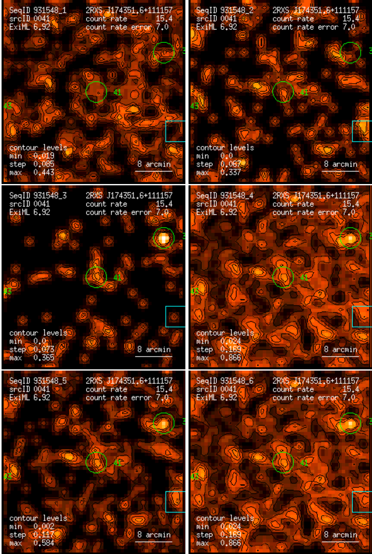
Figure 41: RASS 931548: detection 0041: band rate images, Gaussian filter: (1) PSPC channels 11 – 41, (2) 52 – 90, (3) 91 – 201, (4) 11 – 235, (5) 52 – 201, (6) 11 – 201. Broad band rates in counts/ks. Band rate contour levels in counts/ks/arcmin 2 .
