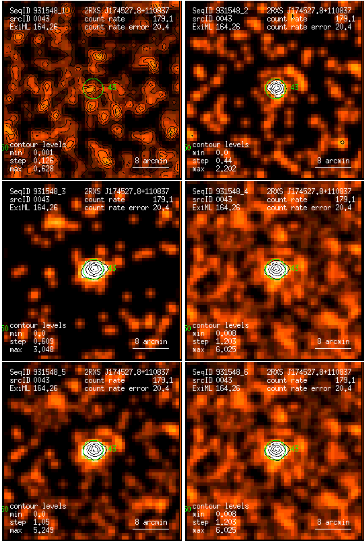
Figure 43: RASS 931548: detection 0043: band rate images, Gaussian filter: (1) PSPC channels 11 – 41, (2) 52 – 90, (3) 91 – 201, (4) 11 – 235, (5) 52 – 201, (6) 11 – 201. Broad band rates in counts/ks. Band rate contour levels in counts/ks/arcmin 2 .
