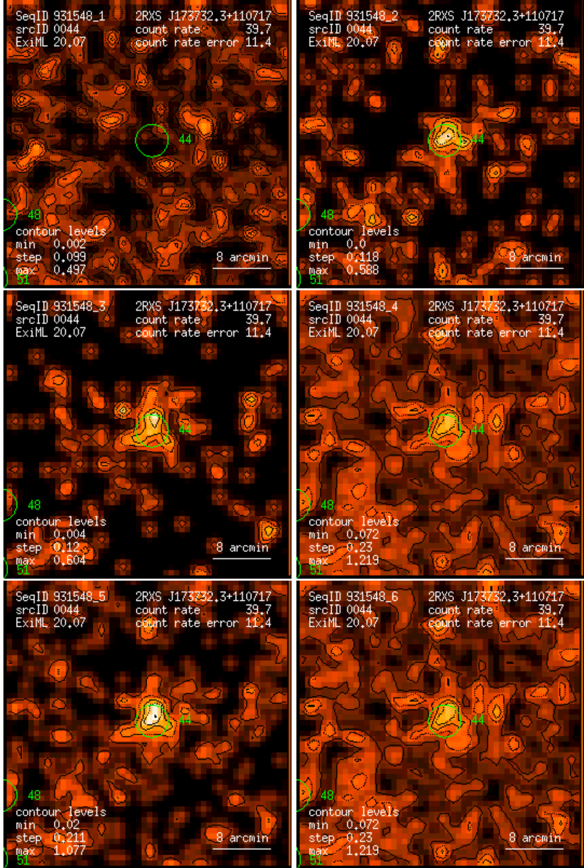
Figure 44: RASS 931548: detection 0044: band rate images, Gaussian filter: (1) PSPC channels 11 – 41, (2) 52 – 90, (3) 91 – 201, (4) 11 – 235, (5) 52 – 201, (6) 11 – 201. Broad band rates in counts/ks. Band rate contour levels in counts/ks/arcmin 2 .
