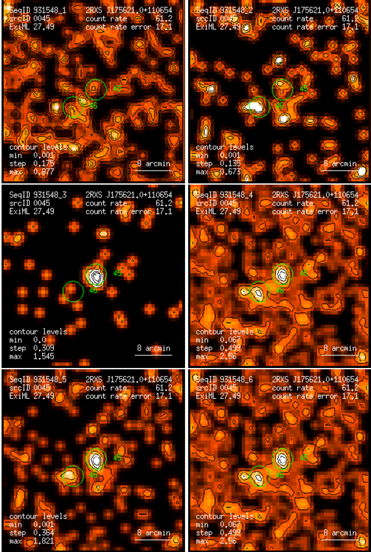
Figure 45: RASS 931548: detection 0045: band rate images, Gaussian filter: (1) PSPC channels 11 – 41, (2) 52 – 90, (3) 91 – 201, (4) 11 – 235, (5) 52 – 201, (6) 11 – 201. Broad band rates in counts/ks. Band rate contour levels in counts/ks/arcmin 2 .
